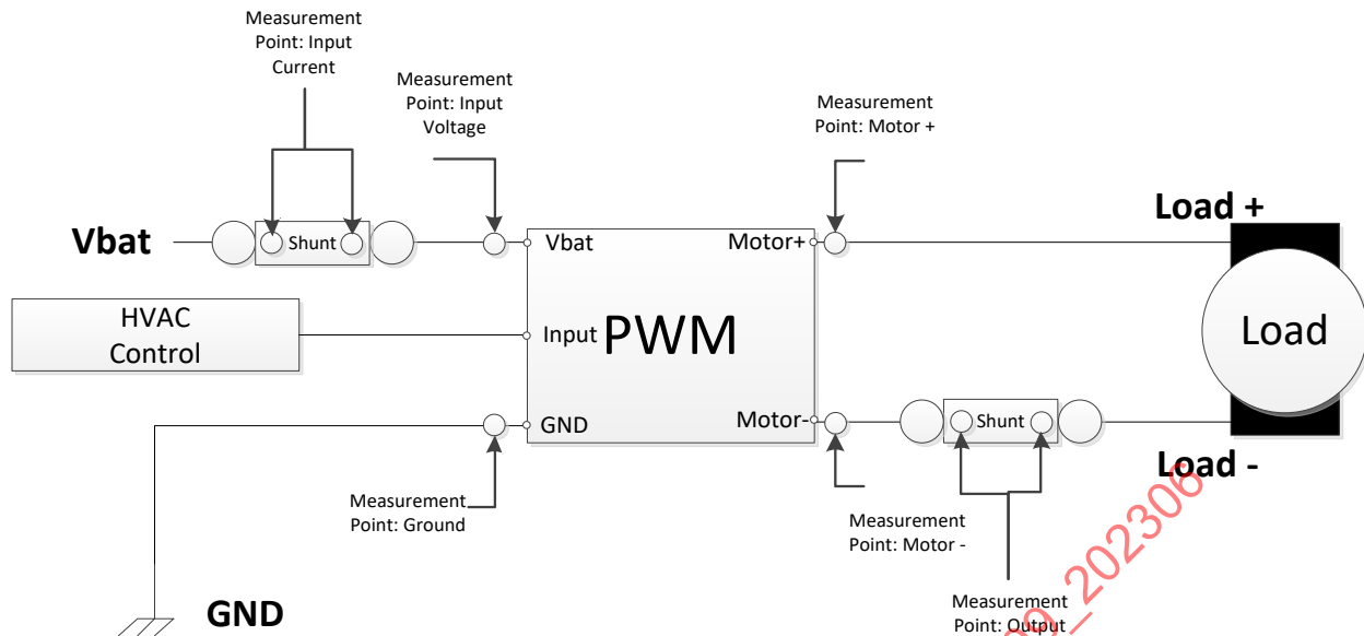
Figure 2 - Test set-up for PWM with high-side switch
