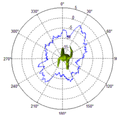
Figure 2 - Measured RCS data of a human subject (173 cm tall and weight 54.4 kg) at walking posture from 360° angles
