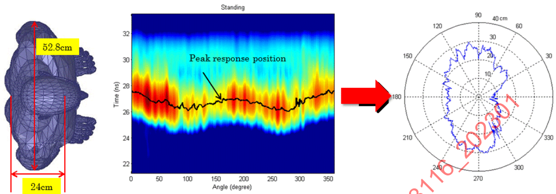
Figure A7 - Simulated 76 to 78 GHz impulse response of a uniformly illuminated male as a function of view angle
