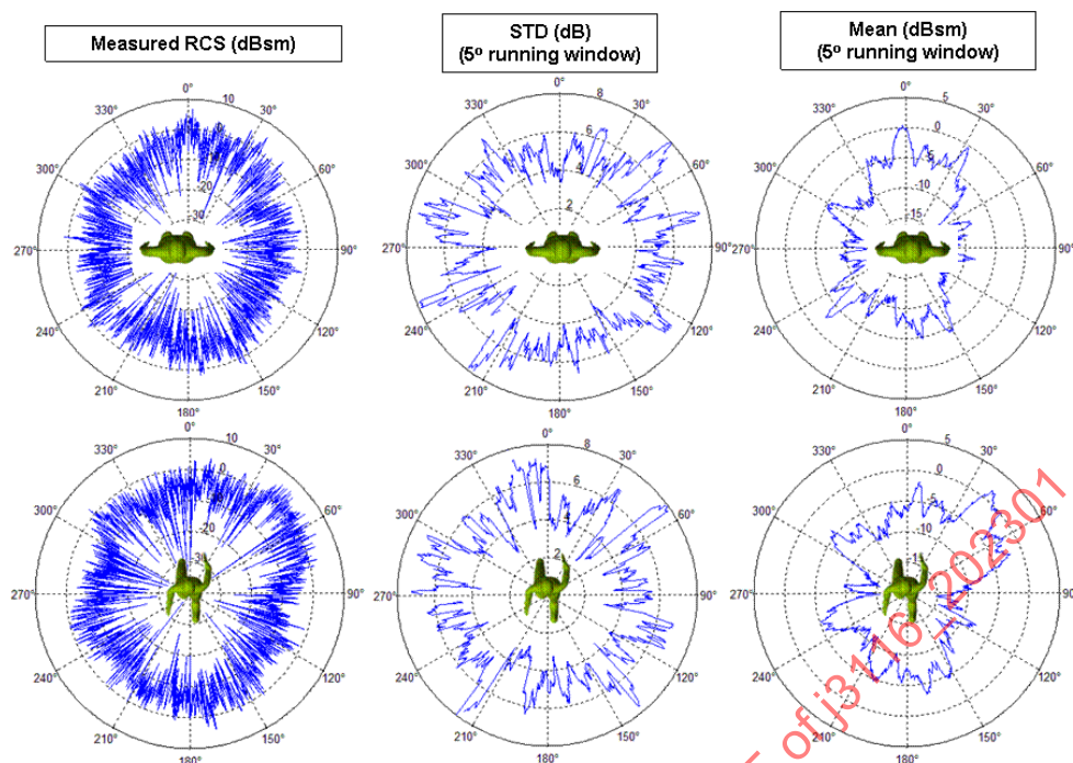
Figure A9 - Measured RCS data for subject #1 - (top) standing posture (bottom) walking posture
