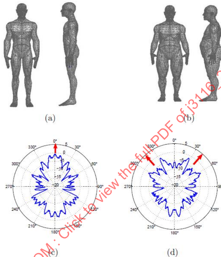
Figure A3 - Comparison of simulated 5° smoothed RCS patterns at 77 GHz between physically fit and obese subjects
