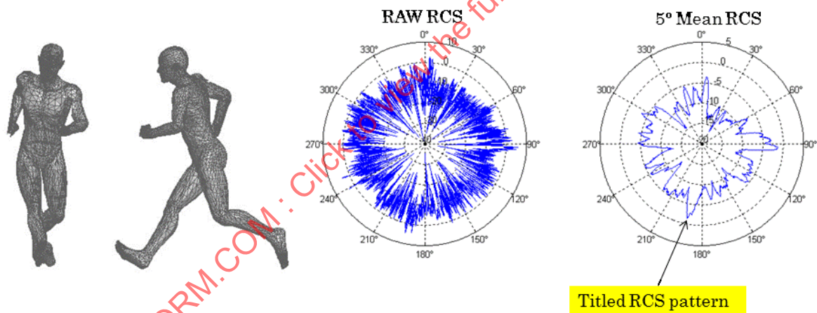
Figure A17 - Simulated RCS patterns of a running adult male
