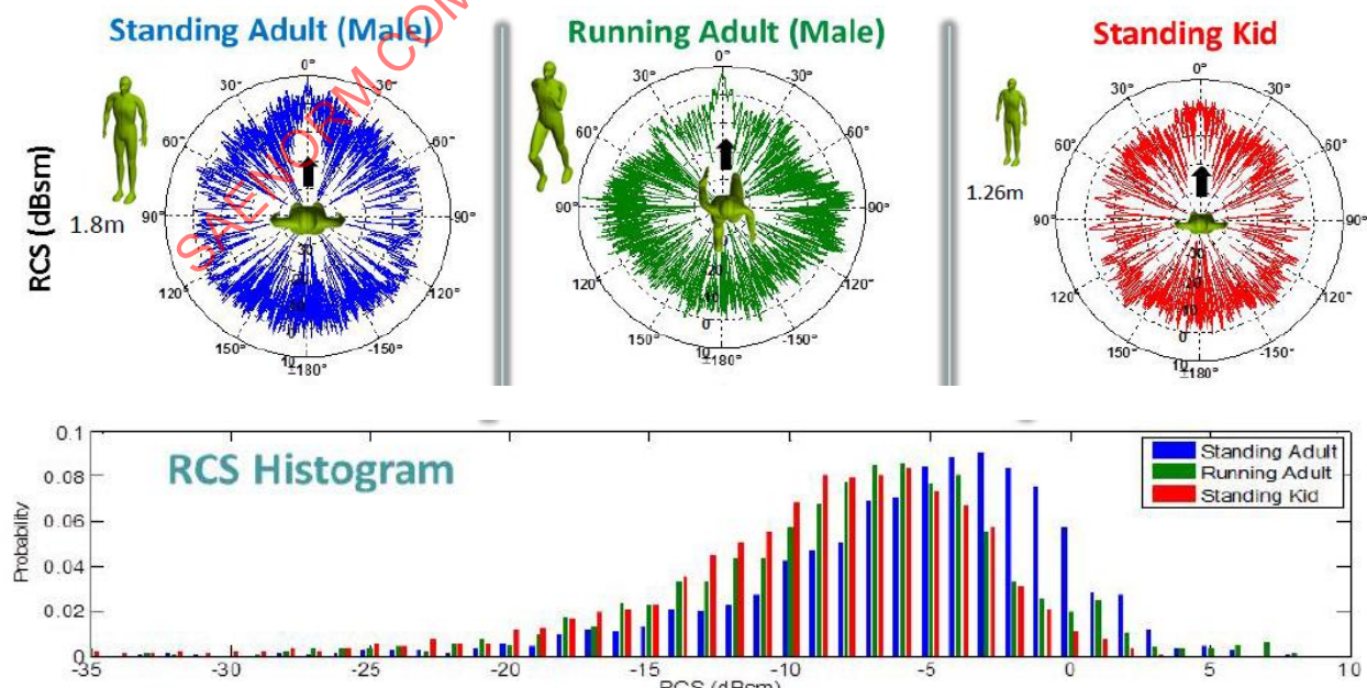
Figure 13 - The numerical model simulated 77 GHz RCS patterns and distributions around 360° of azimuth angles
