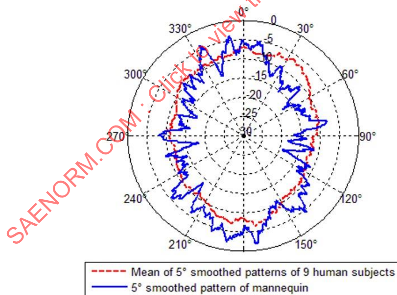
Figure A14 - Comparison between measured 5° smoothed RCS pattern of TASI mannequin and the average of the 5° smoothed RCS pattern of 9 human subjects in standing posture shown in Figure A8
