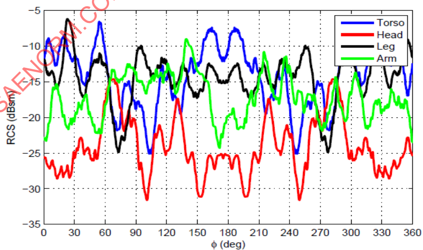
Figure 5 - Simulated 77 GHz scattering from different body parts
