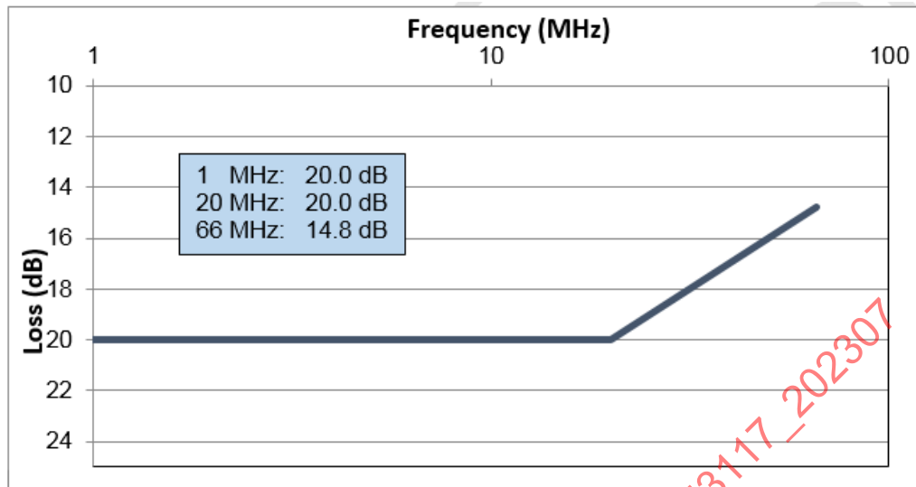
Figure 10 - Return loss requirement
