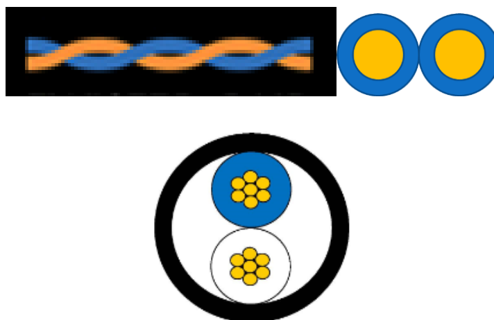
Figure 3 - Un-shielded balanced single twisted pair ethernet cable
