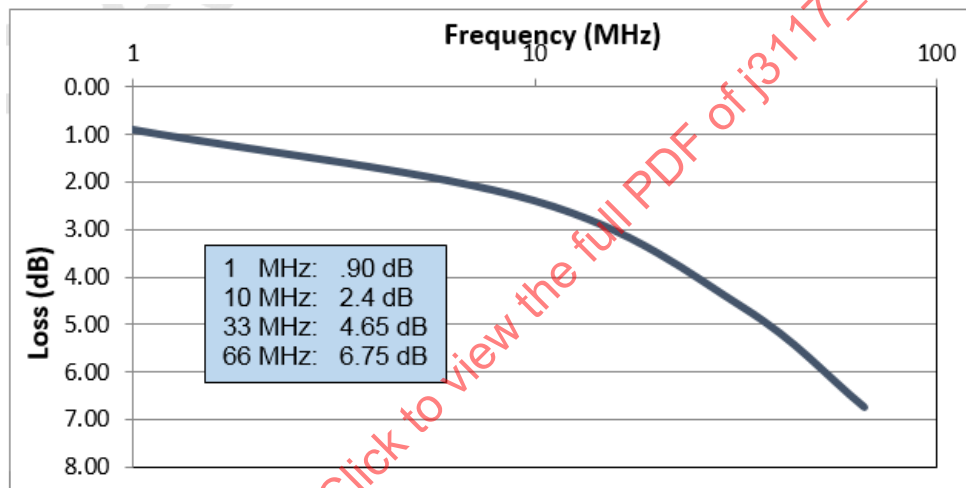
Figure 9 - Insertion loss requirement
