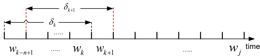
Figure 3 - Sliding window
