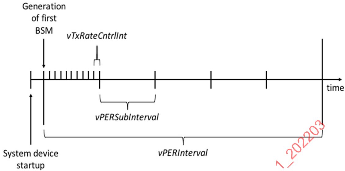
Figure 2 - Relationship between computational intervals: vPERSubInterval , vPERInterval , and vTxRateCntrlInt
