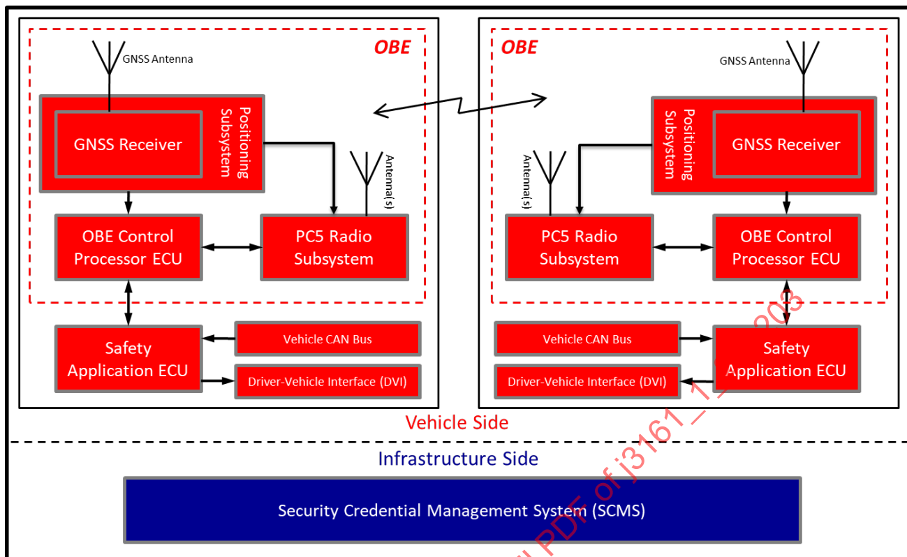
Figure 1 - On-board V2V system
