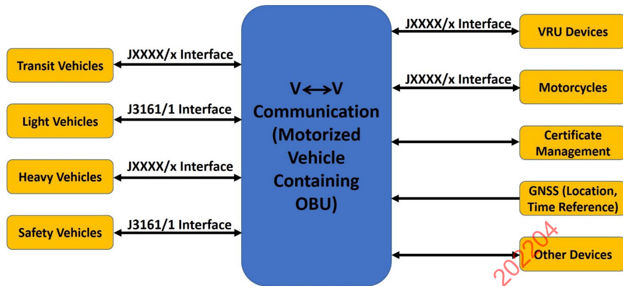
Figure 3 - Vehicle-to-vehicle (V2V) context diagram for LTE-V2X
