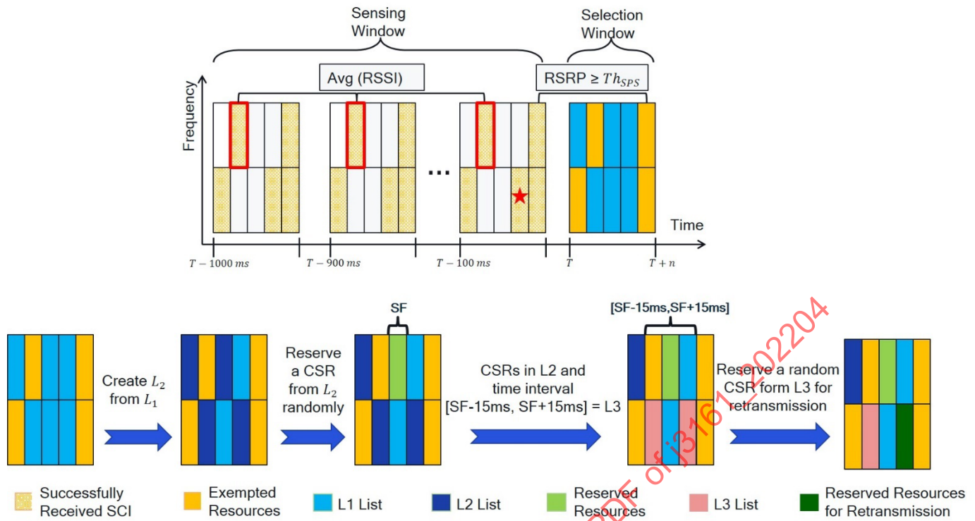
Figure 14 - Illustration of semi-persistent scheduling (SPS) algorithm
