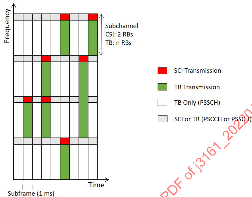
Figure 13 - LTE-V2X sub-channelization
