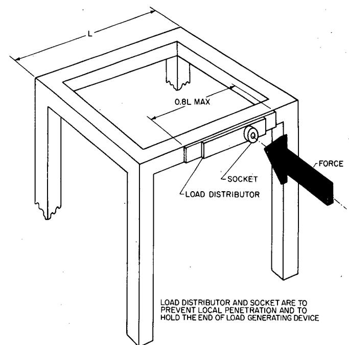
FIG. 5—TYPICAL BUT NOT MANDATORY TEST CONFIGURATION
