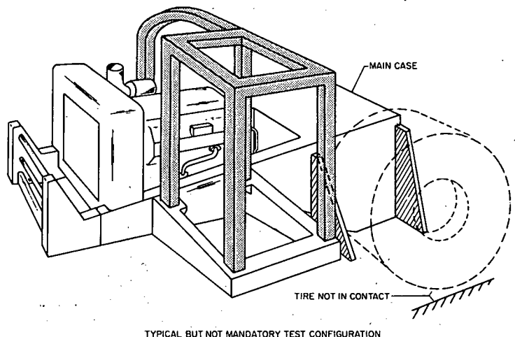
FIG. 2—TYPICAL BUT NOT MANDATORY TEST CONFIGURATION
