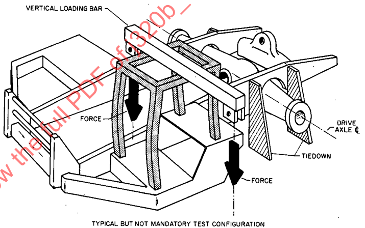
FIG. 4—TYPICAL BUT NOT MANDATORY TEST CONFIGURATION
