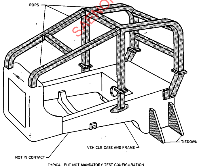
FIG. 1—TYPICAL BUT NOT MANDATORY TEST CONFIGURATION
