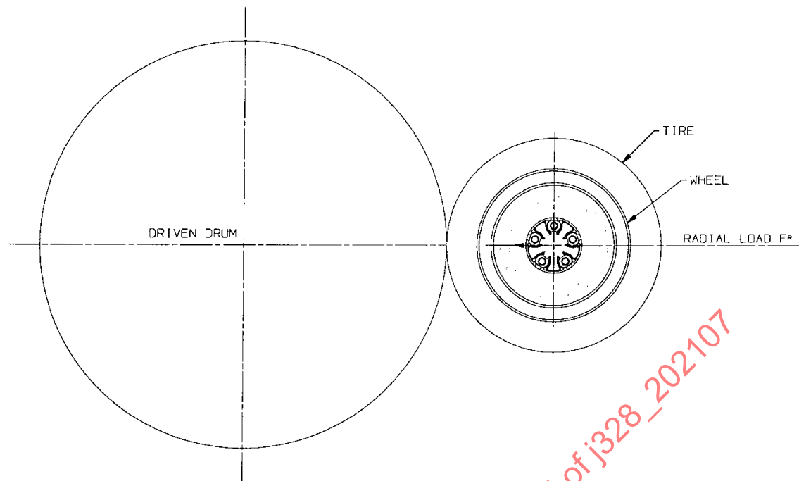
Figure 3 - Radial fatigue (typical set-up)
