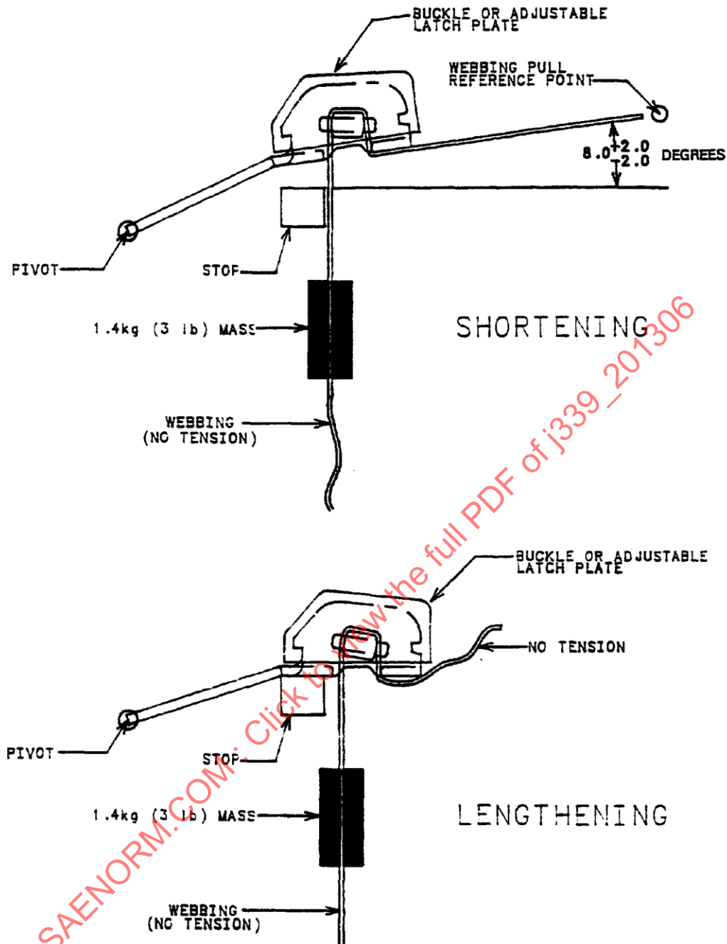
FIGURE 1—WEBBING ABRASION
