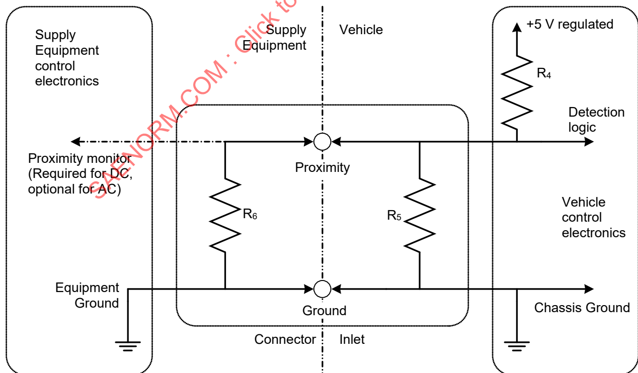
Figure 3 - Simplified case C proximity diagram for SAE J3400 coupler in the Connector Inserted state
