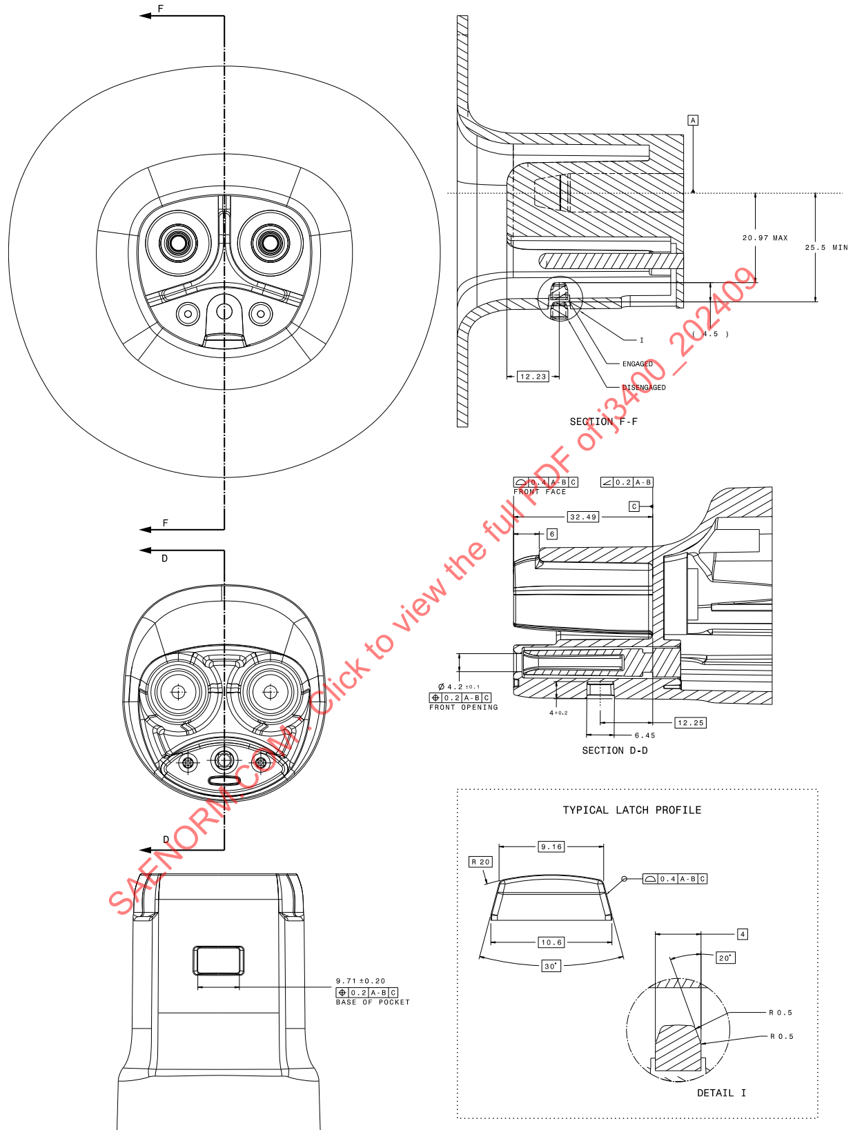
Figure 10 - SAE J3400 latch mechanical drawing
