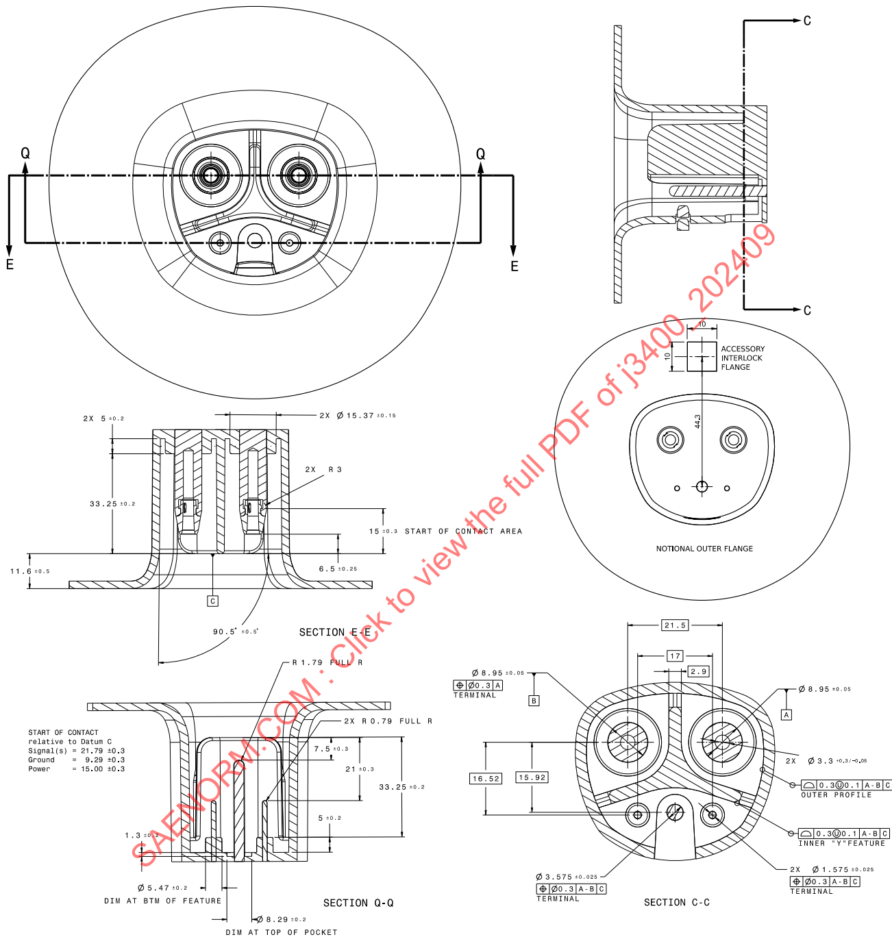
Figure 8 - SAE J3400 inlet mechanical drawing
