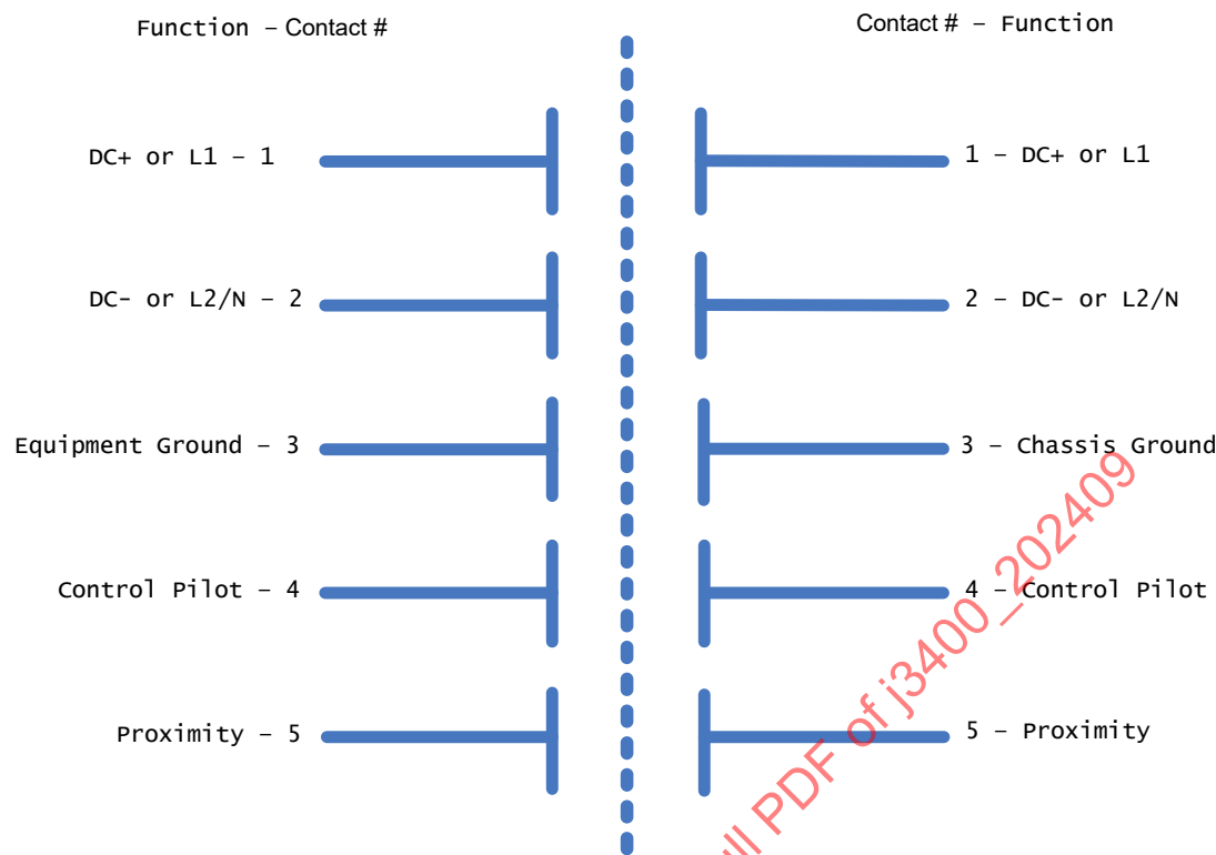
Figure 1 - SAE J3400 coupler conceptual interface: connector (left); inlet (right)
