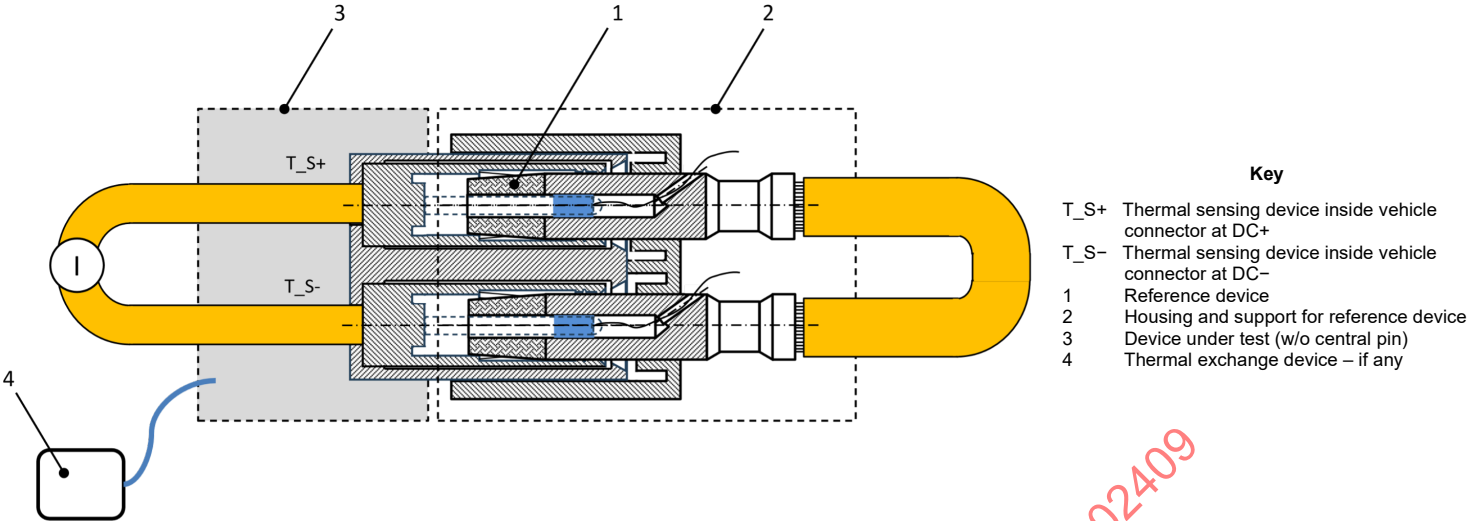
Figure 14 - Mated test setup
