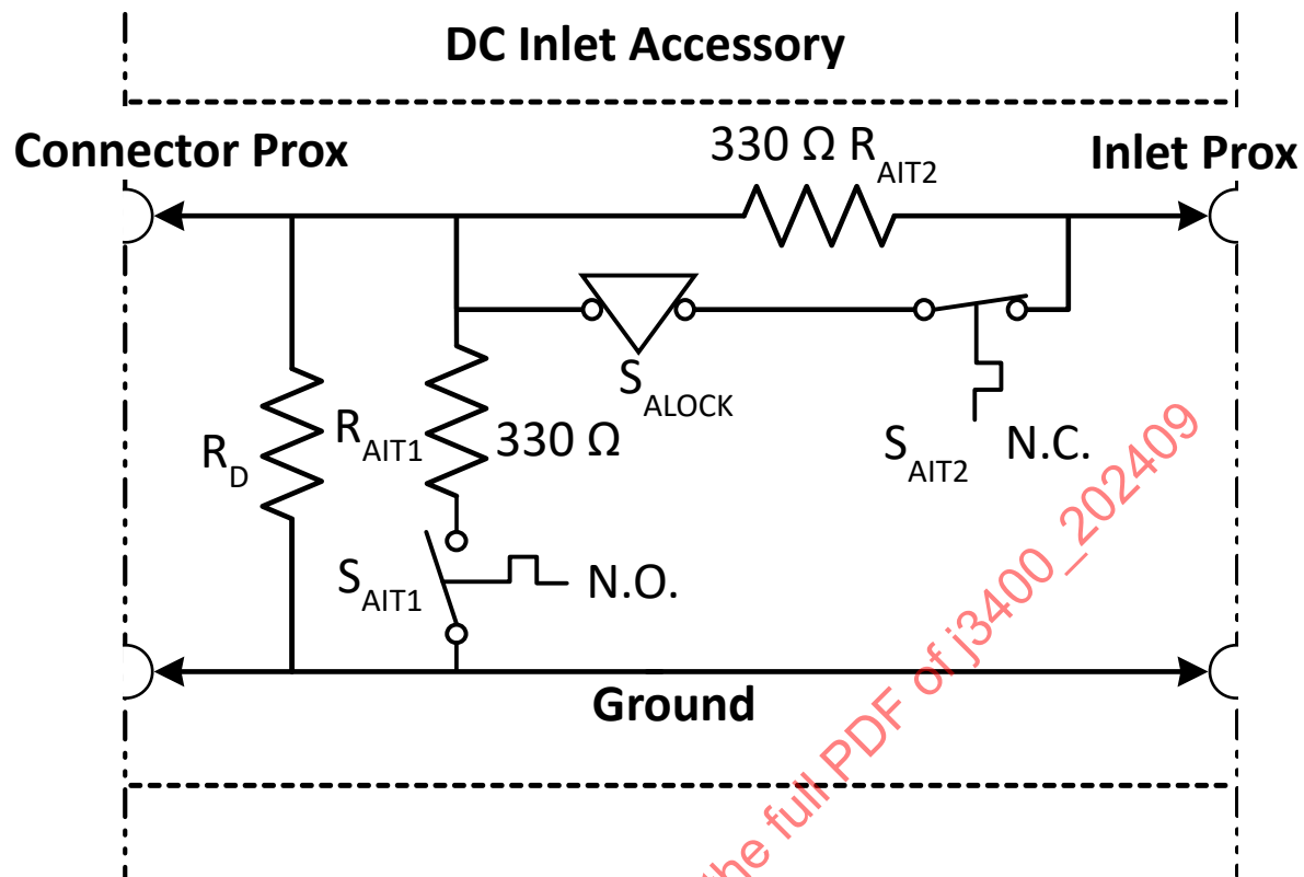
Figure 7 - Inlet accessory with proximity on both mating interfaces typical for DC power transfer from CCS
