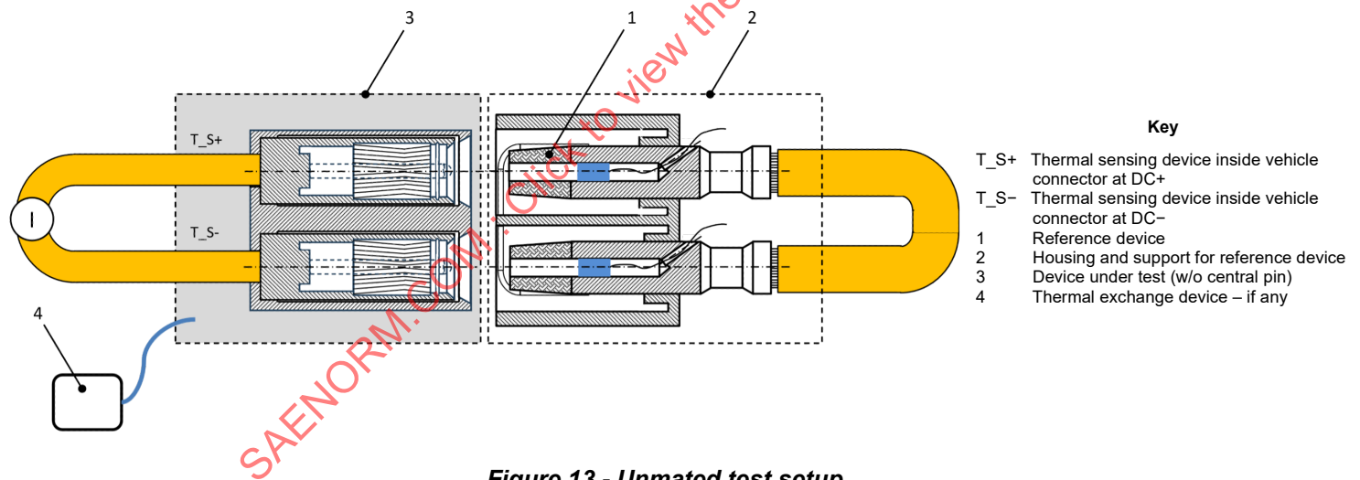
Figure 13 - Unmated test setup
