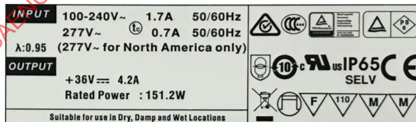
Figure 5 - Example photo of a mixed voltage range rating compliance label (for EU, US/CA, JP, etc.) (informative-use only)
