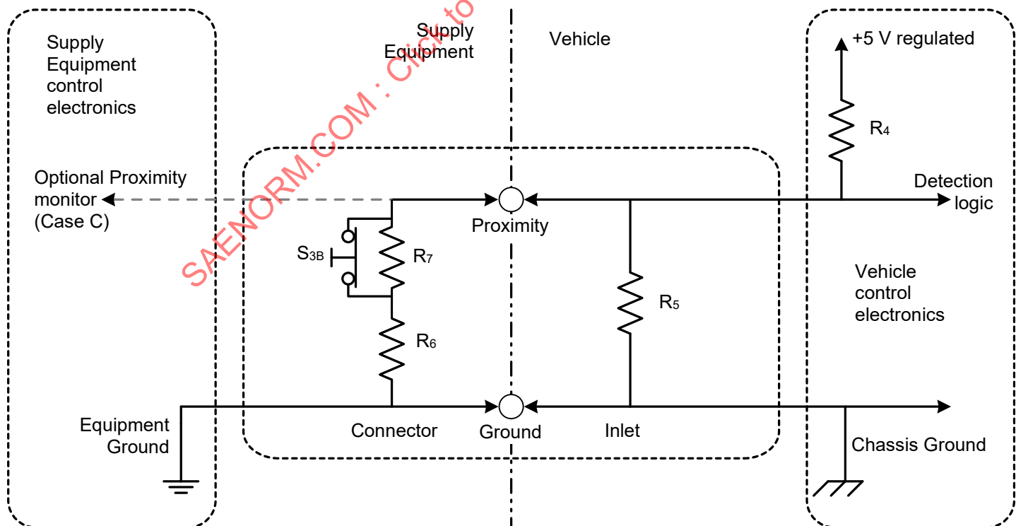
Figure 4 - EV-sensed request-to-stop on SAE J3400 connectors for AC power transfer
