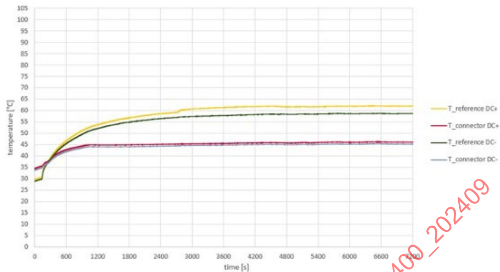
Figure 16 - Example result for temperature rise test. Test is passed.
