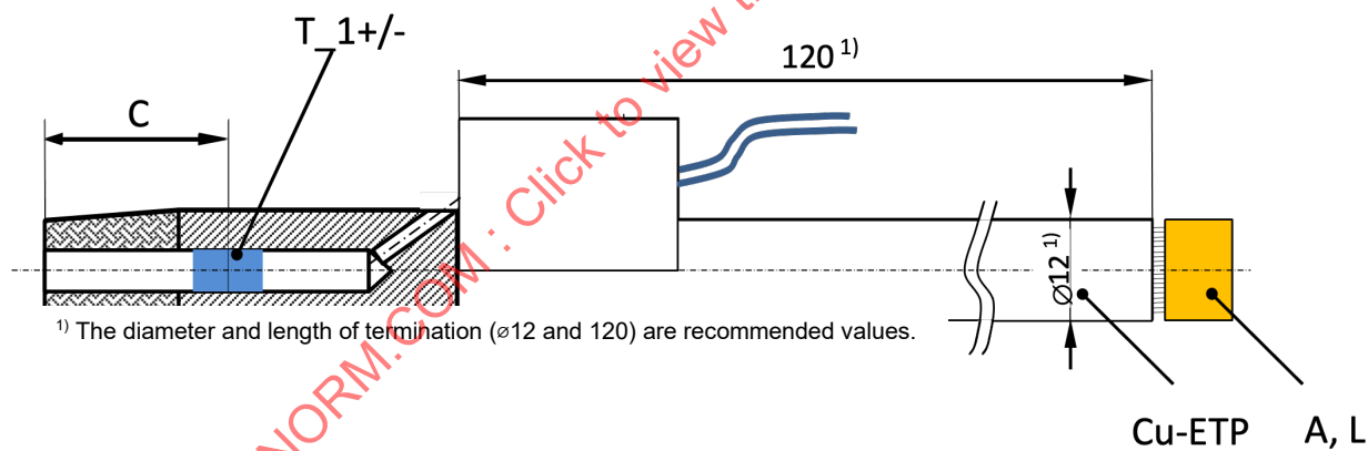
Figure 12 - Reference device with contact dimensions, with heater
