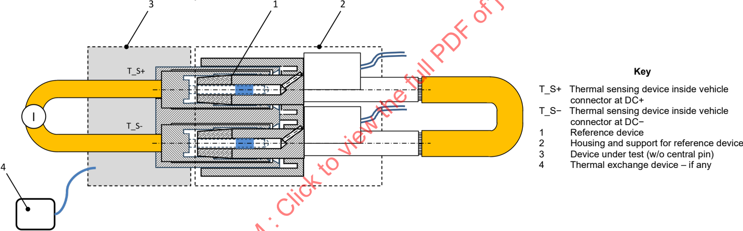
Figure 15 - Test setup with heater
