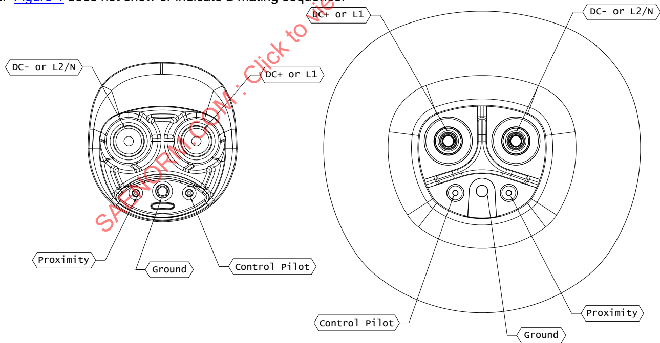
Figure 2 - SAE J3400 coupler mechanical interface: connector (left); inlet (right)
