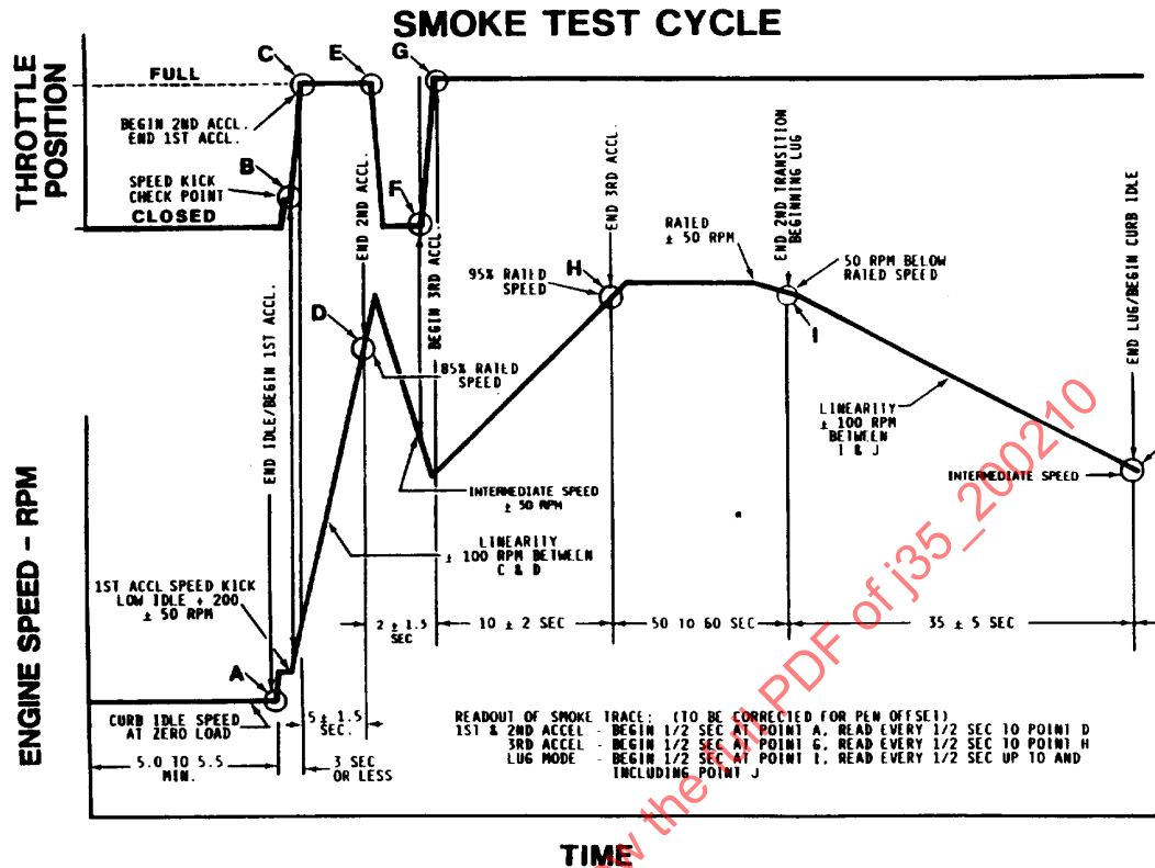
FIGURE 1—SMOKE TEST CYCLE
