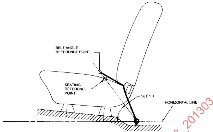
FIGURE 1—BELT OUTSIDE SEAT OR THROUGH SEAT SPRINGS
