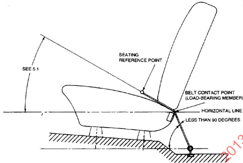
FIGURE 3—BELT OVER SEAT CROSS BAR
