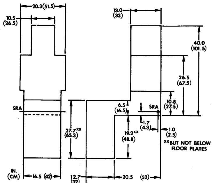
FIG. 2—SEAT REFERENCE POINT
