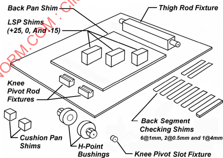
FIGURE C1—CHECKING FIXTURES AND SHIMS
