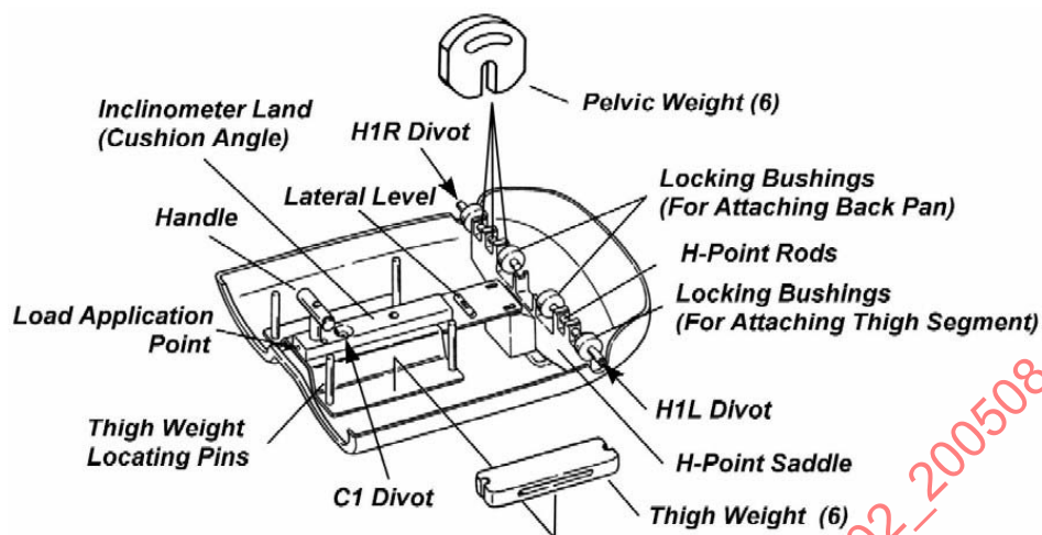
FIGURE 4—CUSHION PAN
