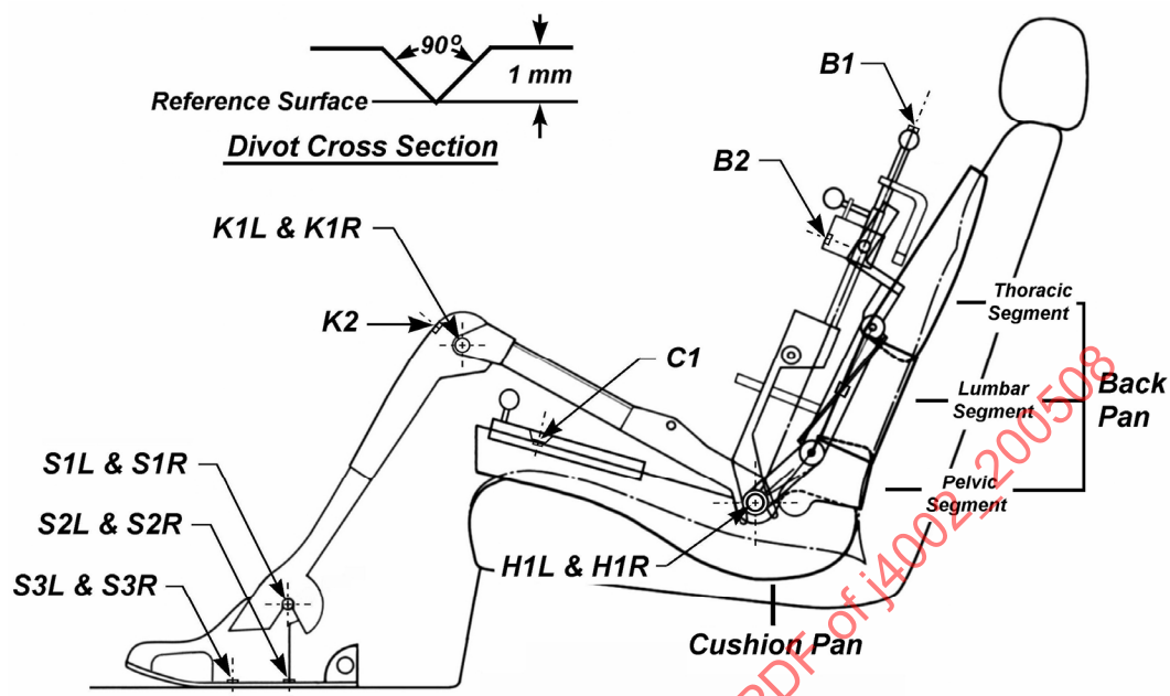
FIGURE C2—HPM REFERENCE POINTS (DIVOT POINTS)
