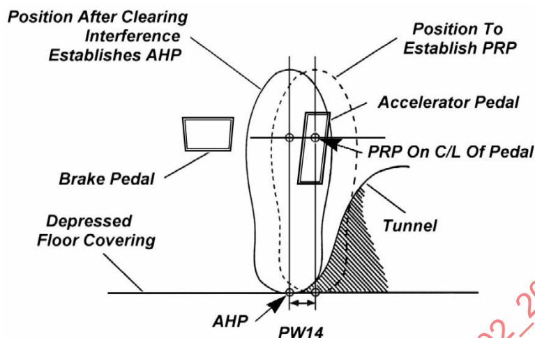
FIGURE 5—AHP TO PRP LATERAL OFFSET
