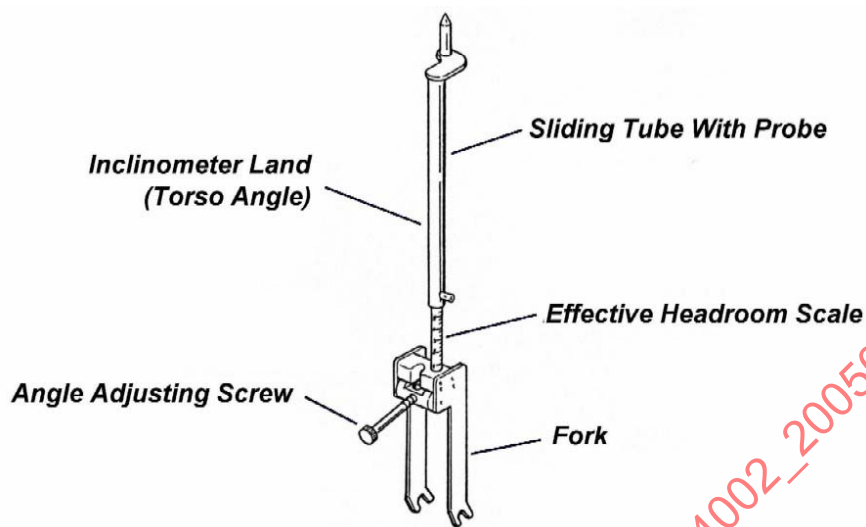
FIGURE 10—HEAD ROOM FIXTURE
