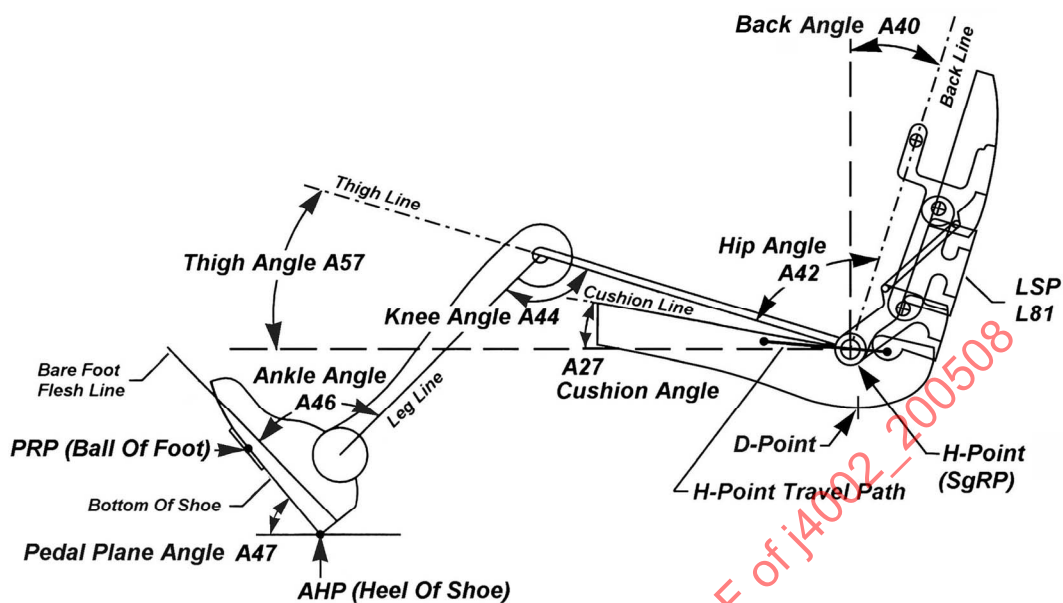
FIGURE A8—REFERENCE POINTS, REFERENCE LINES, AND POSTURE ANGLES
