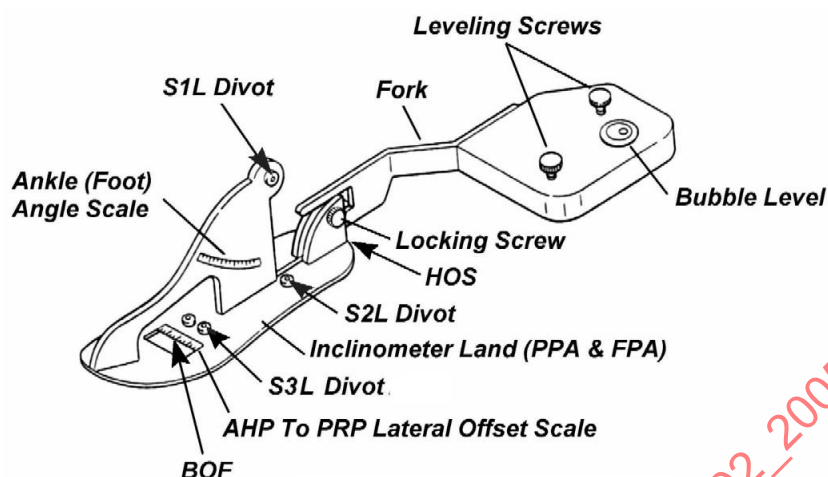
FIGURE A4—SHOE AND SHOE FIXTURE
