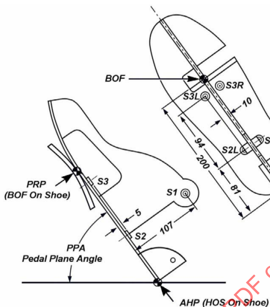
FIGURE 7—SHOE DIVOT POINTS
