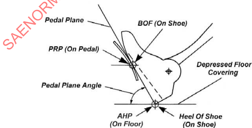
FIGURE 6—SHOE REFERENCE POINTS
