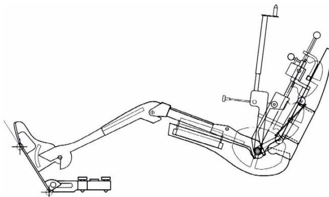
FIGURE 1—SIDE VIEW OF HPM
