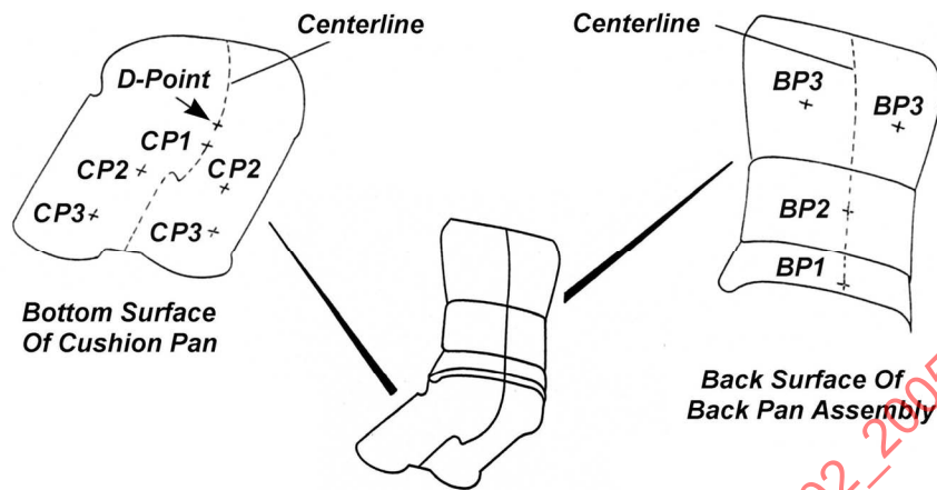
FIGURE A6—SUPPORT POINTS
