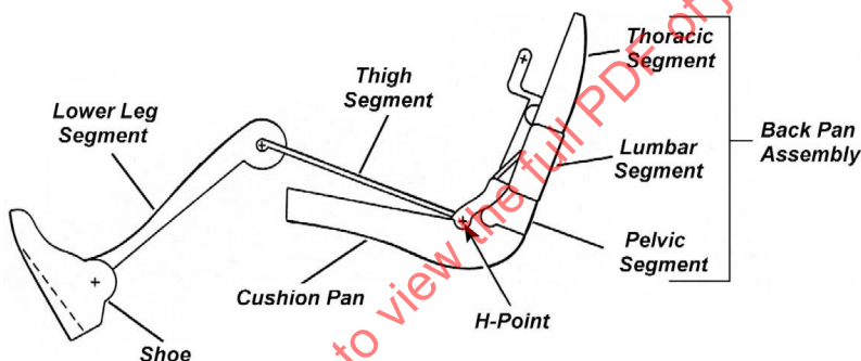
FIGURE A1—MAJOR NEW HPM COMPONENTS
