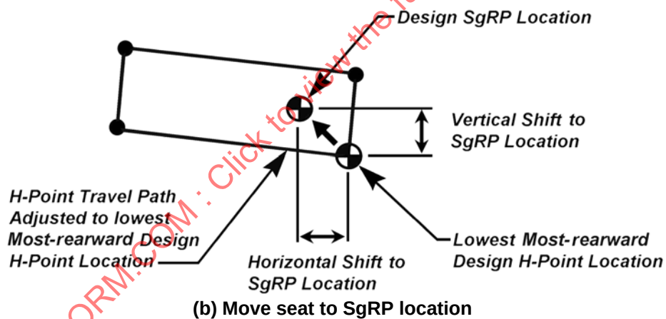
FIGURE 2 - LOCATING SGRP FROM THE SEAT TRAVEL PATH
