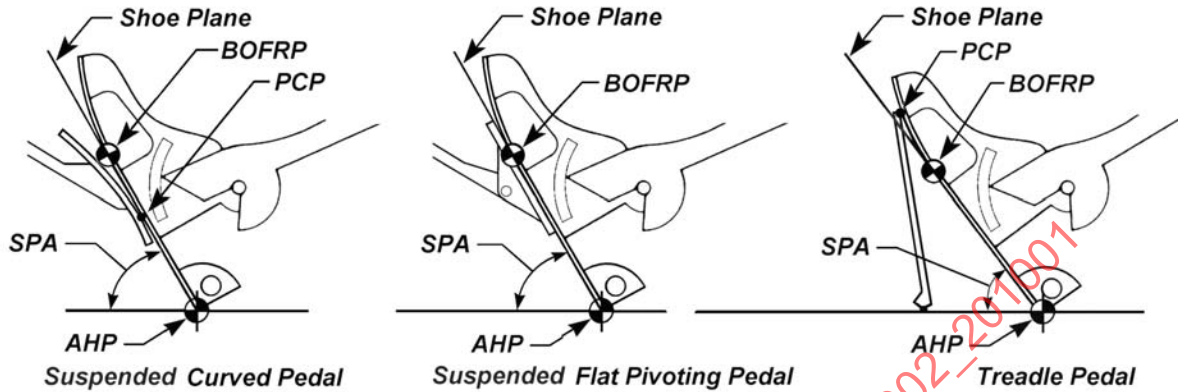
FIGURE 8 - SHOE REFERENCE POINTS RELATED TO ACCELERATOR PEDAL
