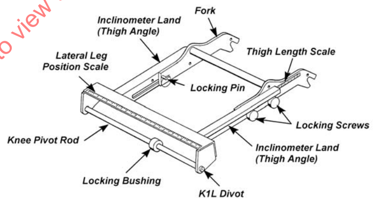
FIGURE A3 - THIGH SEGMENT
