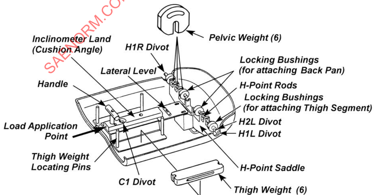
FIGURE 4 - CUSHION PAN
