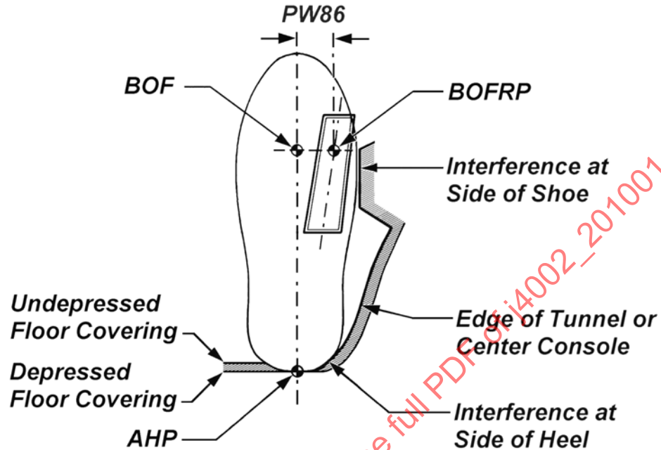
FIGURE 6 - AHP TO BOFRP LATERAL OFFSET
