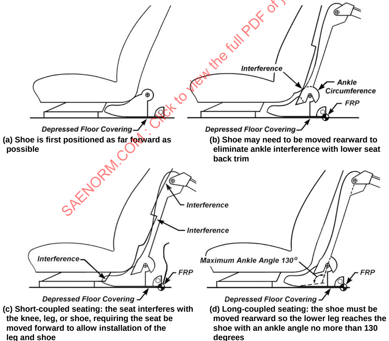
FIGURE 10 - SHOE AND LEG INSTALLATION FOR REAR PASSENGER SEATS
