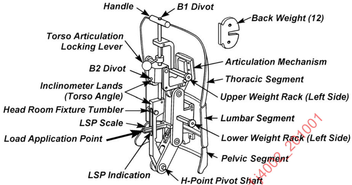
FIGURE 3 - BACK PAN
