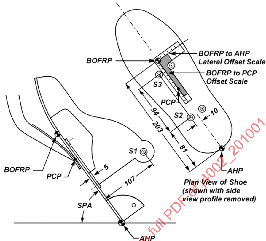
FIGURE 9 - SHOE DIVOT POINTS
