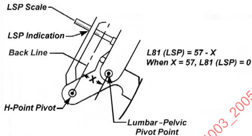
FIGURE 2—LUMBAR SUPPORT PROMINENCE (LSP)
