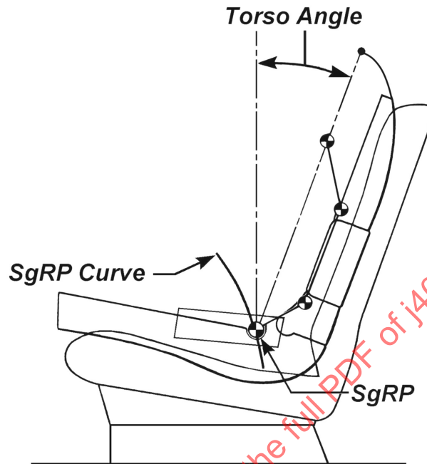
FIGURE 8 - DESIGN TORSO ANGLE OF HPD IS SET BY MANUFACTURER
