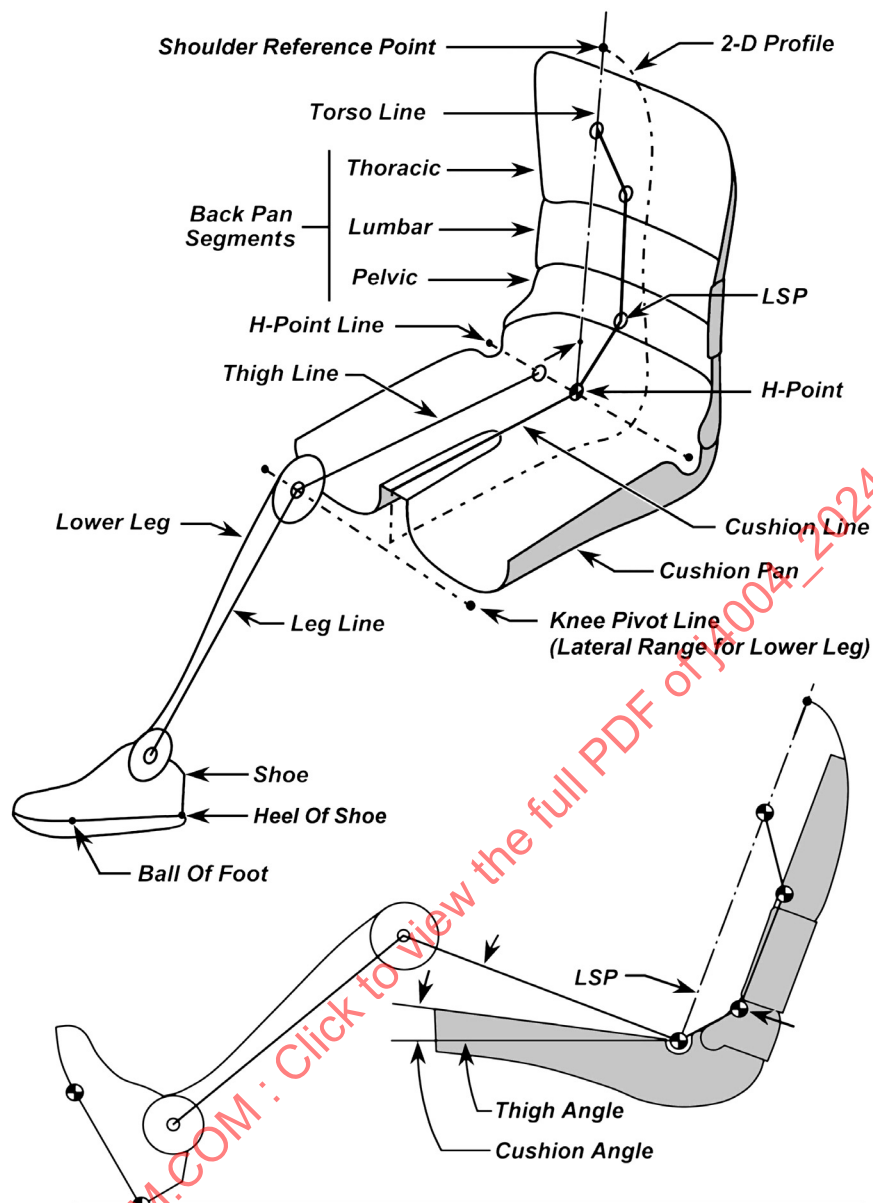
FIGURE 2 - H-POINT DESIGN TOOL (HPD) - ELEMENTS ARE COMMON WITH H-POINT MACHINE (HPM-II) EXCEPT FOR PARTS OF THE 2-D PROFILE
