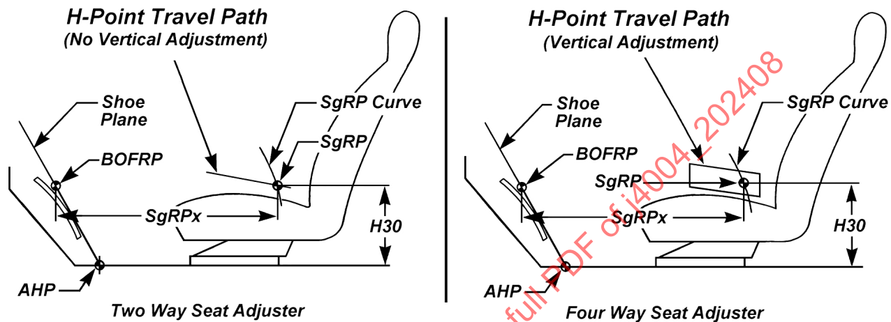
FIGURE 6 - H-POINT TRAVEL PATHS, 2-WAY AND 4-WAY SEAT ADJUSTER
