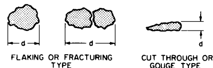
FIG. 3—CHIP SIZE MEASUREMENT APPROXIMATION
