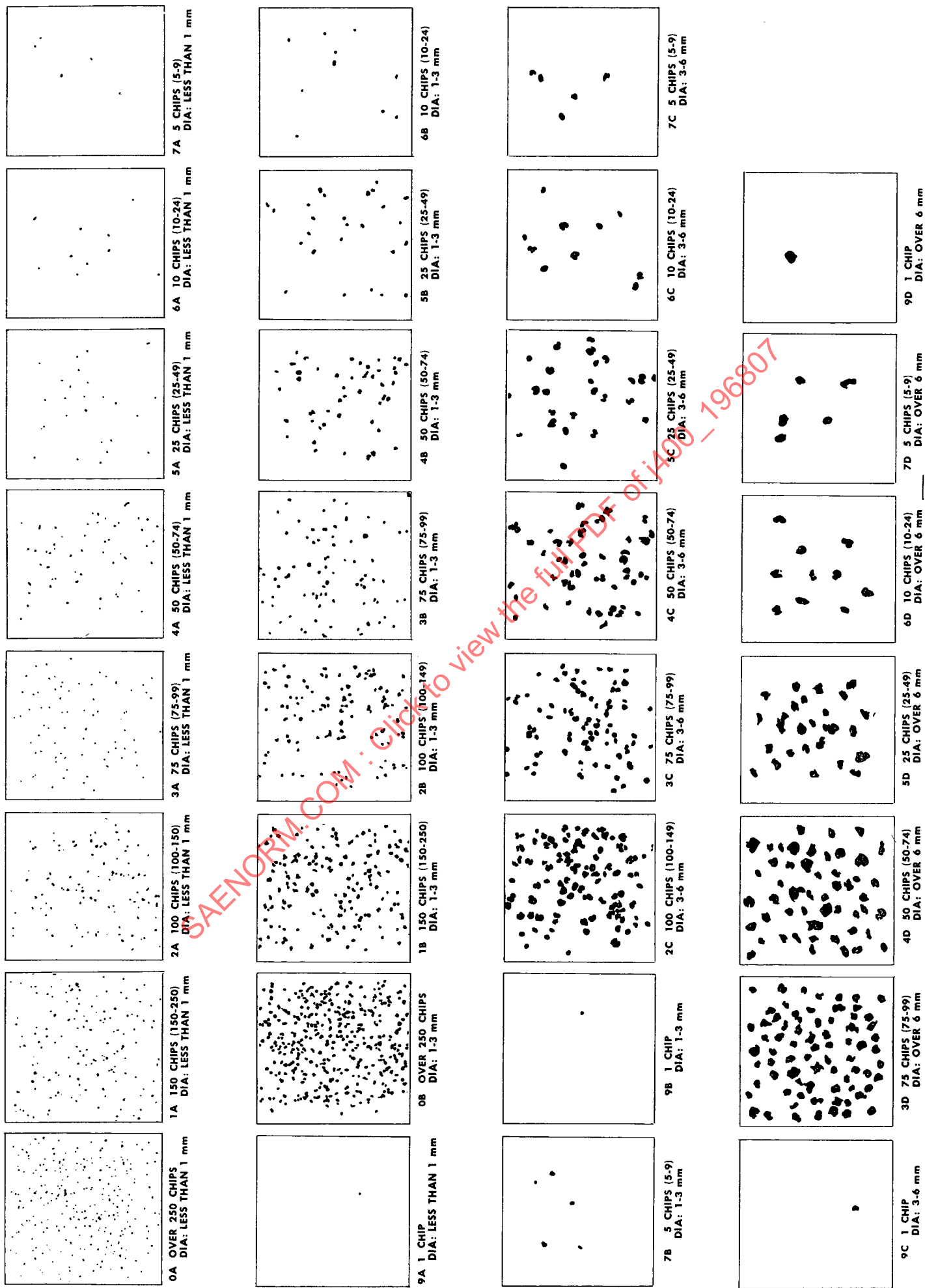
FIG. 2—CHIPPING RATING STANDARDS (REPRESENTATION ONLY)
