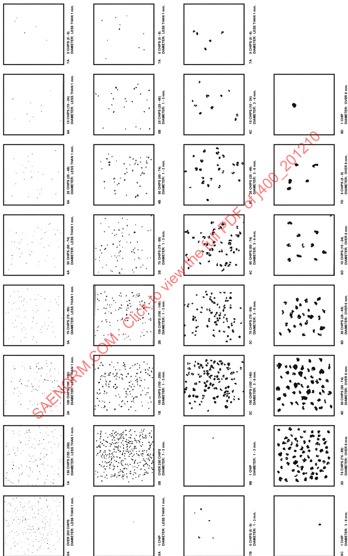
FIGURE 3 – CHIPPING RATING STANDARDS (REPRESENTATION ONLY)
