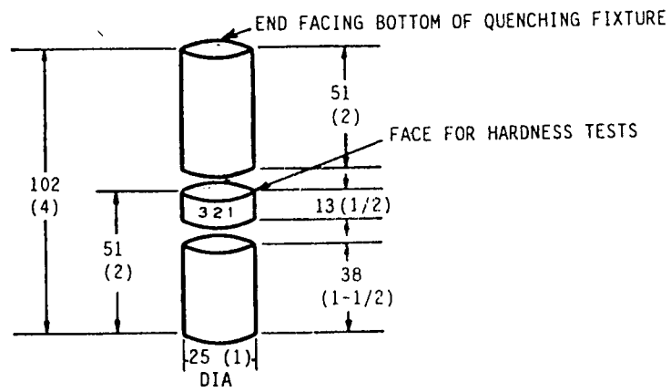
FIGURE 10—LOCATION OF TEST SLUG AND OF STAMPED IDENTIFICATION
