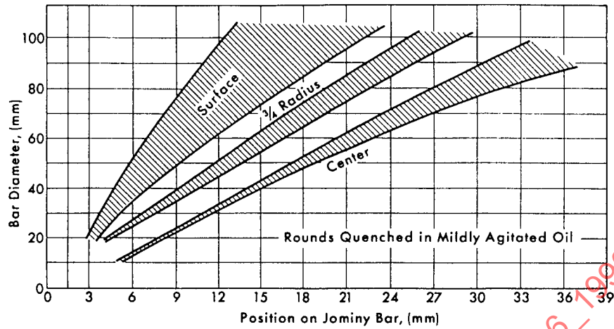
FIGURE 7B—CORRELATION OF COOLING RATES IN JOMINY BAR AND QUENCHED ROUND BARS
