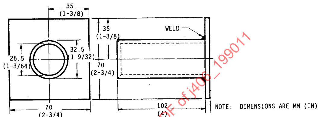
FIGURE 4—HARDENING BAR PROTECTING FIXTURE TO BE CONSTRUCTED OF HEAT RESISTING ALLOY
