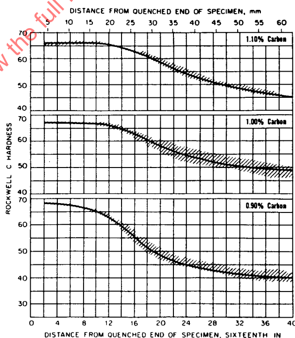
FIGURE A2—REPRODUCIBILITY OF CASE HARDENABILITY
