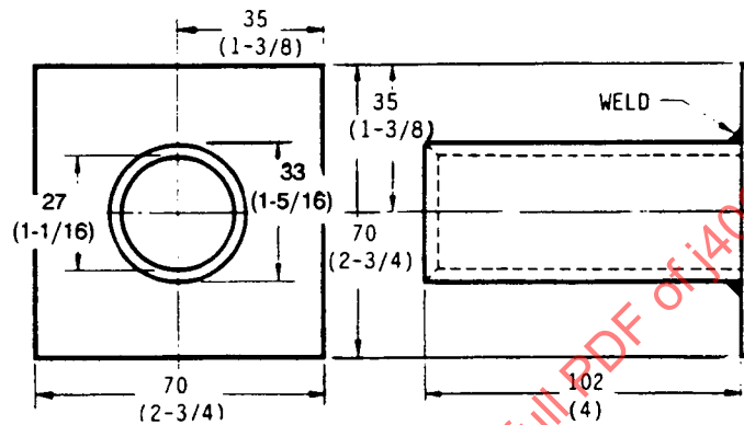
FIGURE 4—HARDENING BAR PROTECTING FIXTURE TO BE CONSTRUCTED OF HEAT-RESISTING ALLOY
