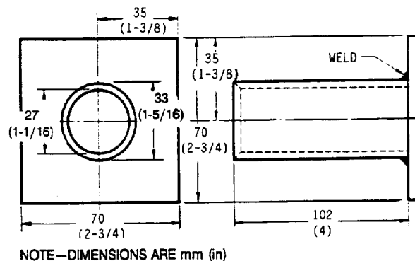
FIGURE 4—SPECIMEN PROTECTING FIXTURE TO BE CONSTRUCTED OF HEAT-RESISTING ALLOY
