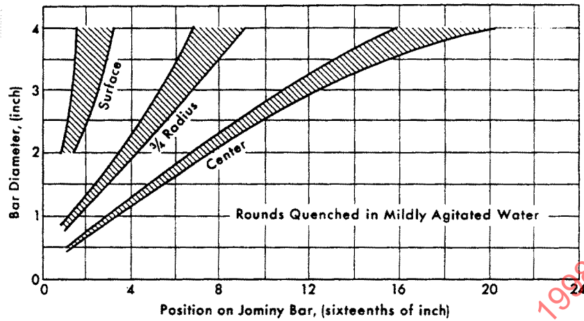
FIGURE 7C—CORRELATION OF COOLING RATES IN JOMINY BAR AND QUENCHED ROUND BARS
