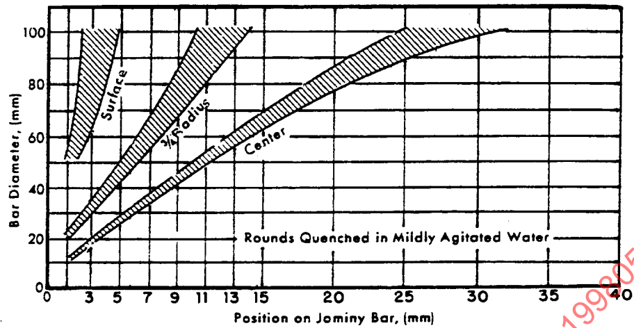
FIGURE 7A—CORRELATION OF COOLING RATES IN JOMINY BAR AND QUENCHED ROUND BARS
