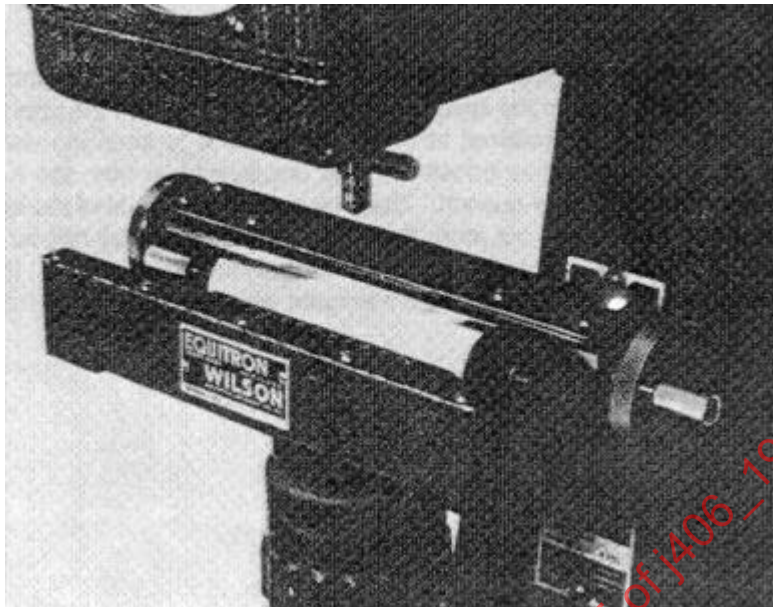
FIGURE 5—COMMERCIALY AVAILABLE FIXTURE FOR POSITIONING SPECIMEN FOR HARDNESS INDENTATIONS
