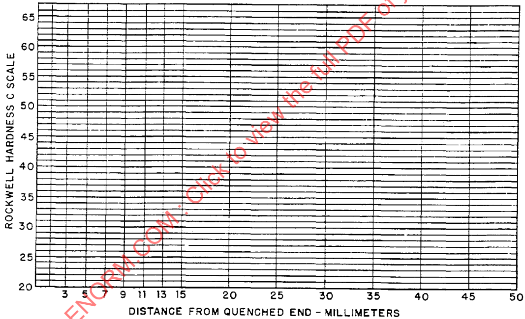
FIGURE 6A—STANDARD FORM FOR PLOTTING HARDENABILITY CURVES (MILLIMETER DISTANCES)
