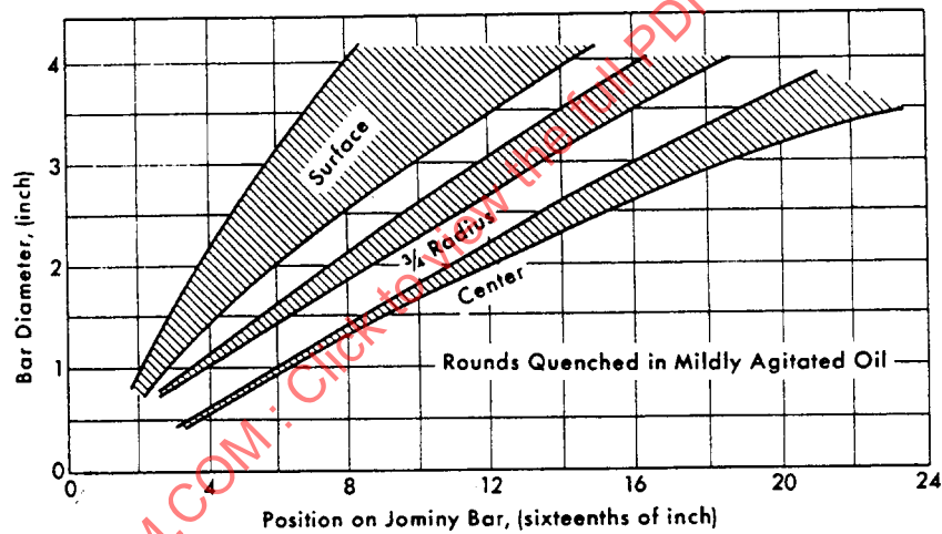
FIGURE 7D—CORRELATION OF COOLING RATES IN JOMINY BAR AND QUENCHED ROUND BARS
