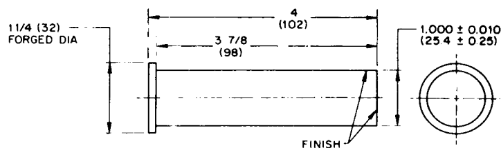
FIG. 2—PREFERRED TEST SPECIMEN
