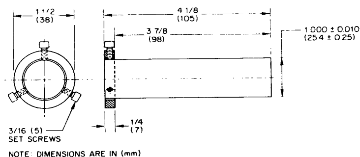
FIG. 3—OPTIONAL TEST SPECIMEN
