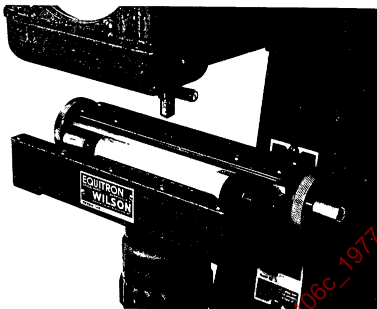
FIG. 5—COMMERCIALLY AVAILABLE FIXTURE FOR POSITIONING SPECIMEN FOR HARDNESS INDENTATIONS
