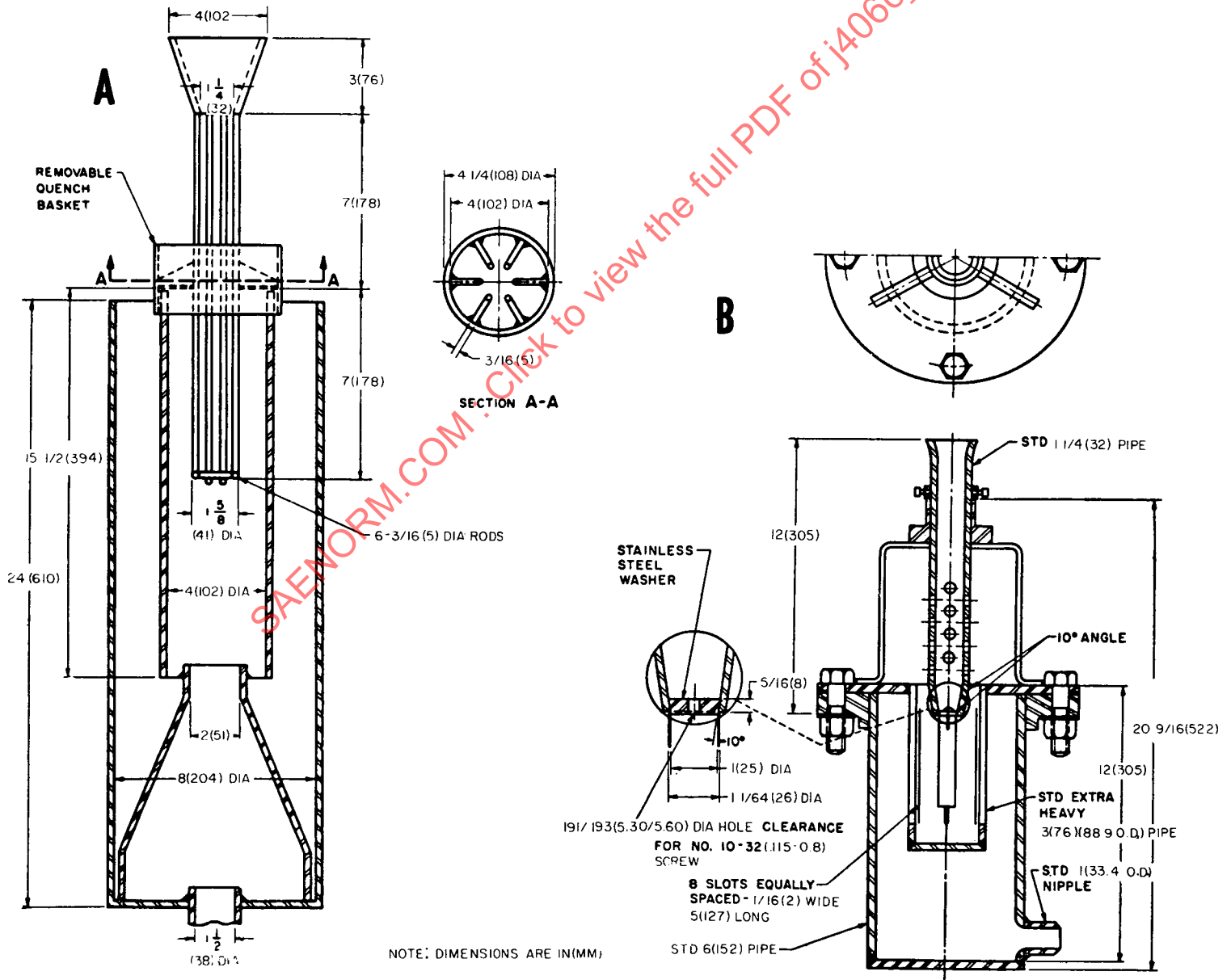
FIG. 9-SAC QUENCHING FIXTURES
