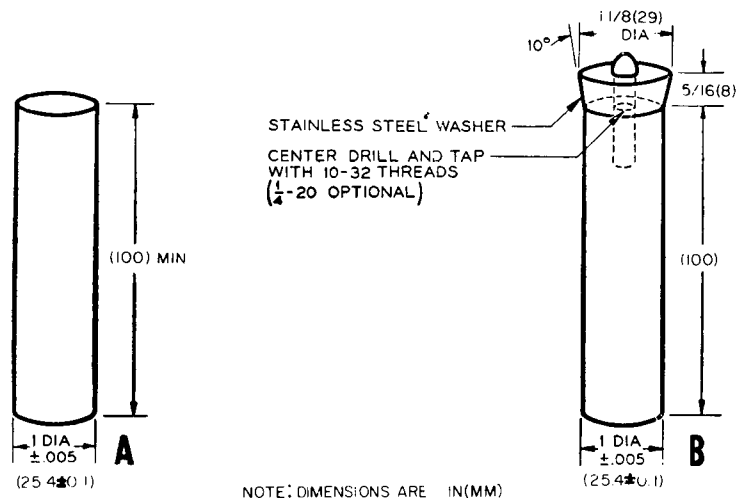
FIG. 8-SAC TEST SPECIMENS
