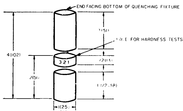
FIG. 10—LOCATION OF TEST SLUG AND OF STAMPED IDENTIFICATION
