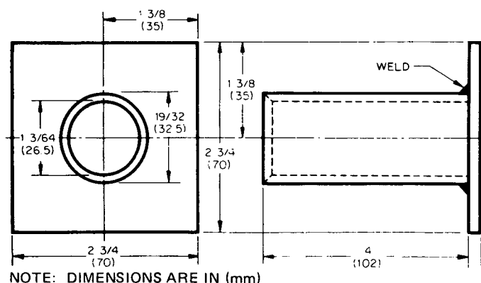
FIG. 4—HARDENING BAR PROTECTING FIXTURE TO BE CONSTRUCTED OF HEAT RESISTING ALLOY
