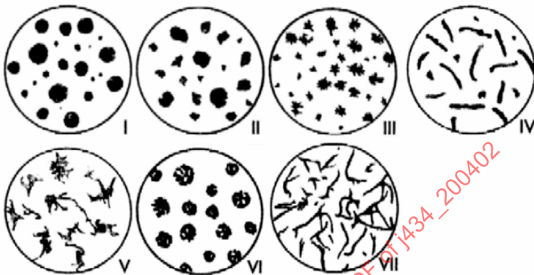
FIGURE 1—CLASSIFICATION OF GRAPHITE SHAPE IN CAST IRONS (FROM ASTM A 247)
