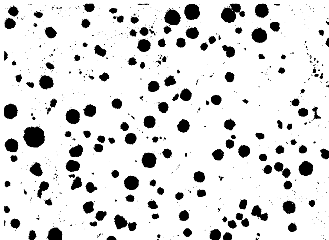
FIG. 3 - D4018, APPROXIMATE 156 BHN (100X) TYPICAL MICROSTRUCTURES
