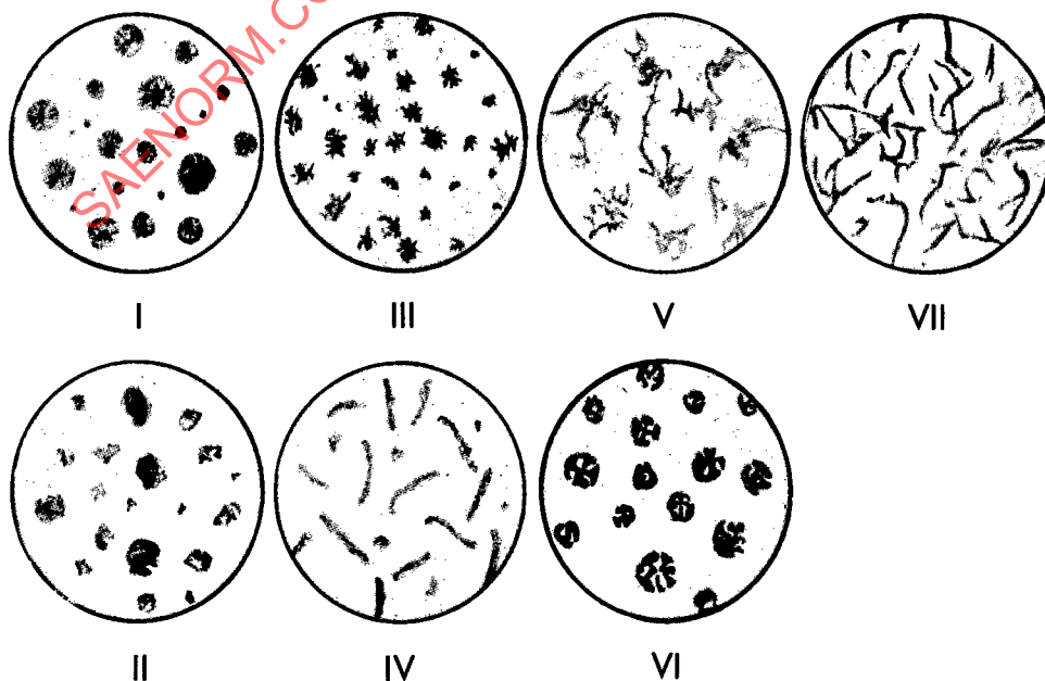
FIG. 1 - CLASSIFICATION OF GRAPHITE SHAPE IN CAST IRONS (FROM ASTM A 247)
