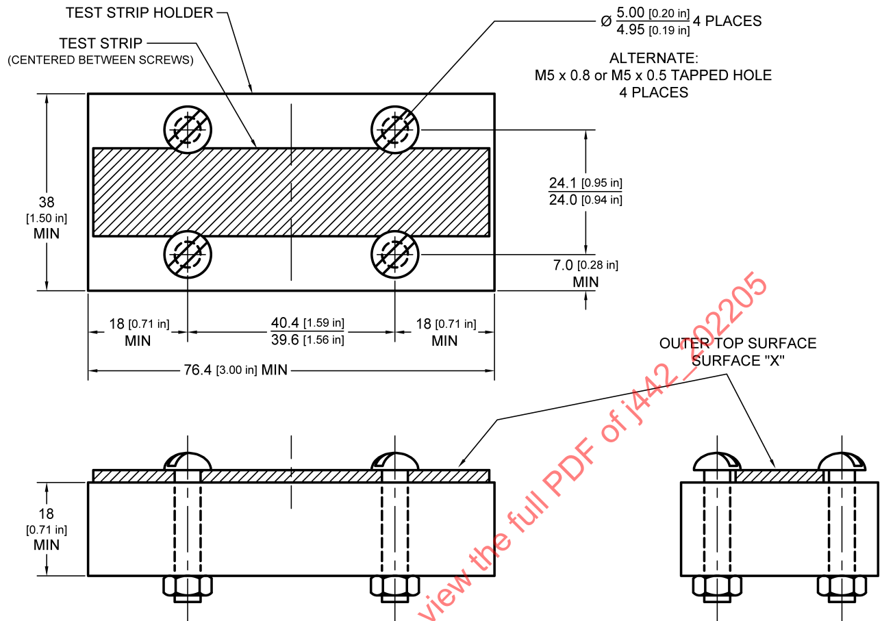
Figure 2 - Assembled standard size strip holder
