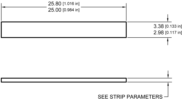
Figure 1B - Sub-size test strip
