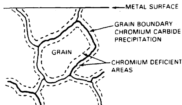
FIGURE 7—INTERGRANULAR CORROSION AT GRAIN BOUNDARIES DUE TO CHROMIUM DEFICIENCY
