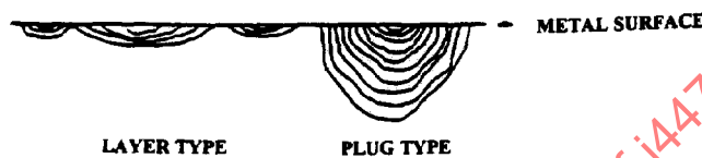
FIGURE 8—DEZINCIFICATION OF BRASS ALLOYS
