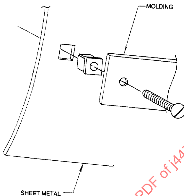
FIGURE 16—FASTENERS
