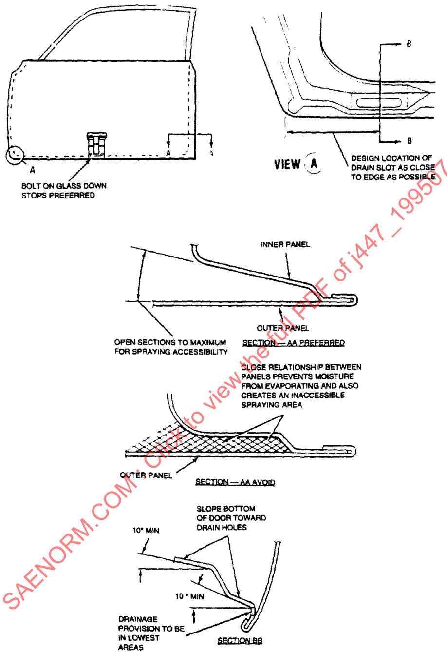
FIGURE 11—DOOR
