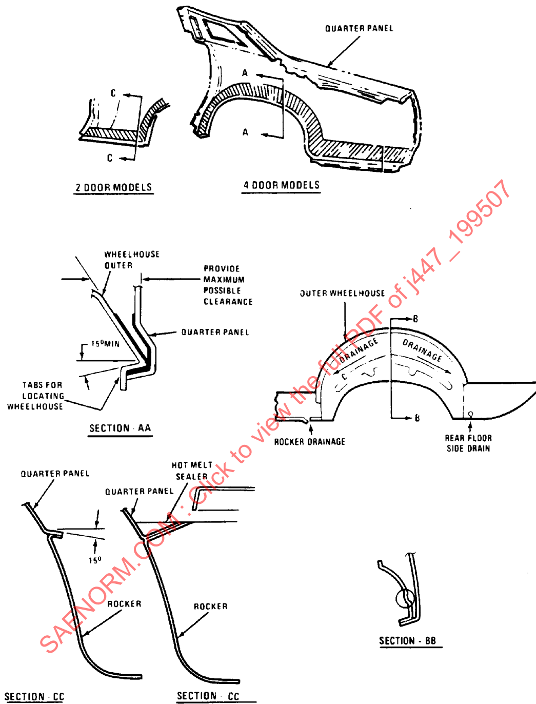
FIGURE 12—QUARTER PANEL ASSEMBLY
