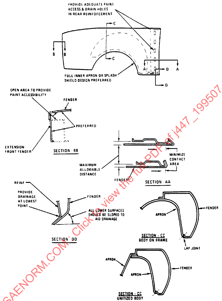
FIGURE 10—FENDER
