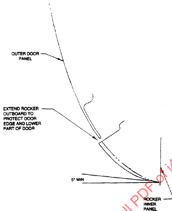
FIGURE 15—ROCKER PANEL
