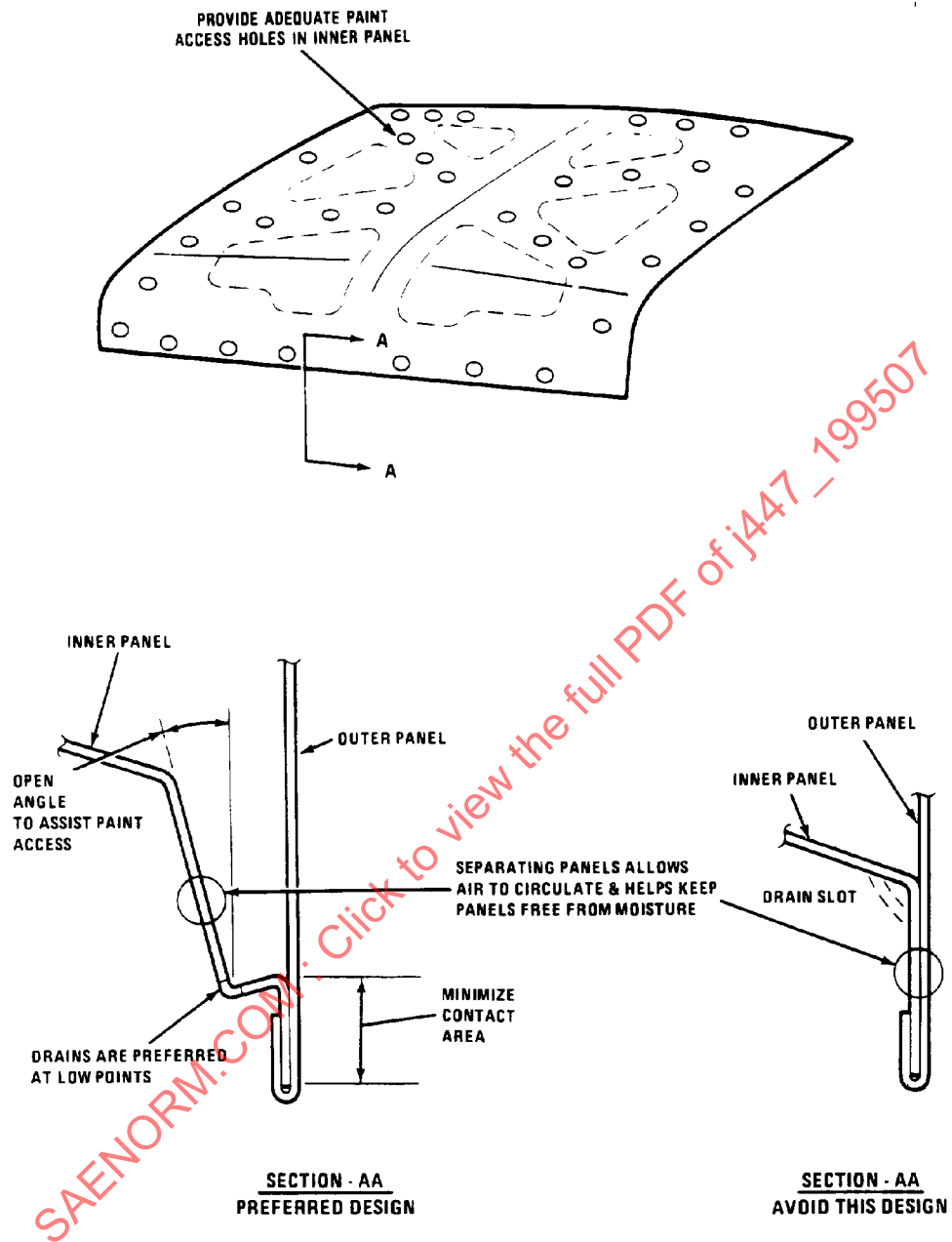
FIGURE 13—DECK LID
