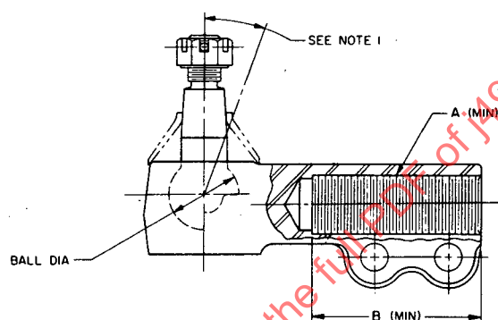
FIG. 4 - TYPICAL BALL STUD SOCKET ASSEMBLY WITH INTERNAL THREADED STEM
