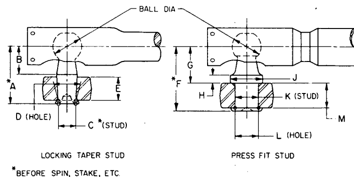
FIG. 6 - TYPICAL TUBULAR ("HORIZONTAL TYPE") SOCKET ASSEMBLY FOR RIVETED, SPUN, STAKED, WELDED, OR THREADED TAPER STUD ATTACHMENT. (FOR THREADED TAPER STUDS, USE TABLE 1 DIMENSIONS)
