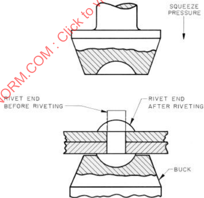
FIGURE A2—SQUEEZE RIVETING
