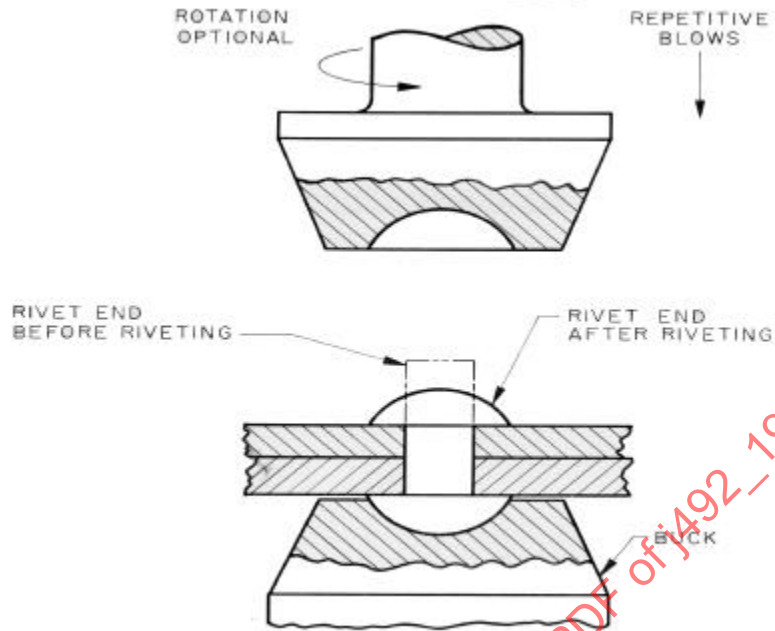
FIGURE A1—IMPACT RIVETING
