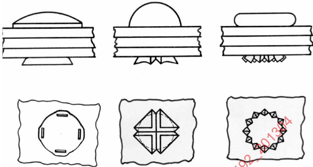
ENDS OF RIVETS
