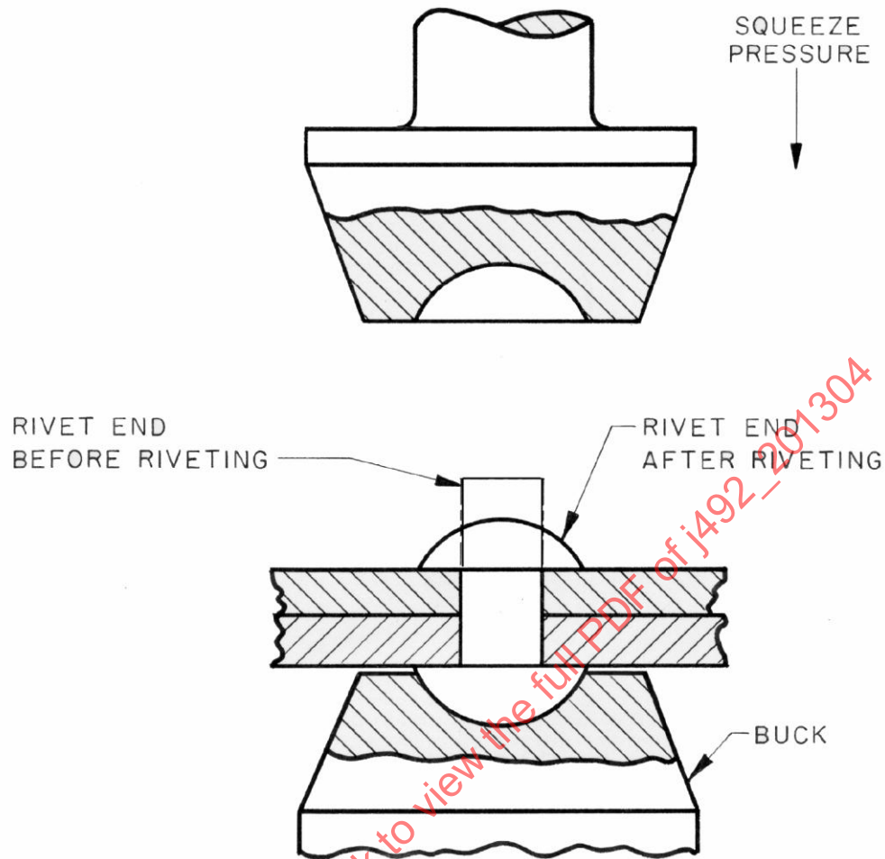
FIGURE 2—SQUEEZE RIVETING
