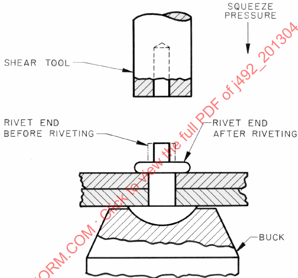
FIGURE 4—SHEAR RIVETING
