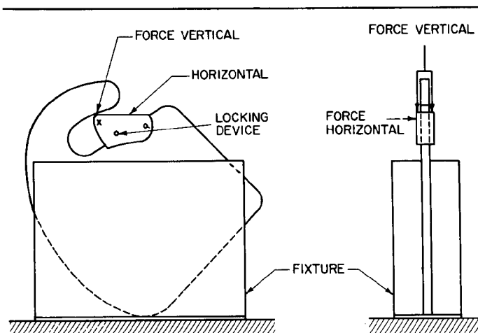
Fig. 4 - Single attachment hook
