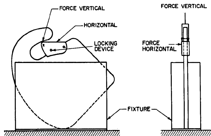
Fig. 4 - Single attachment hook
