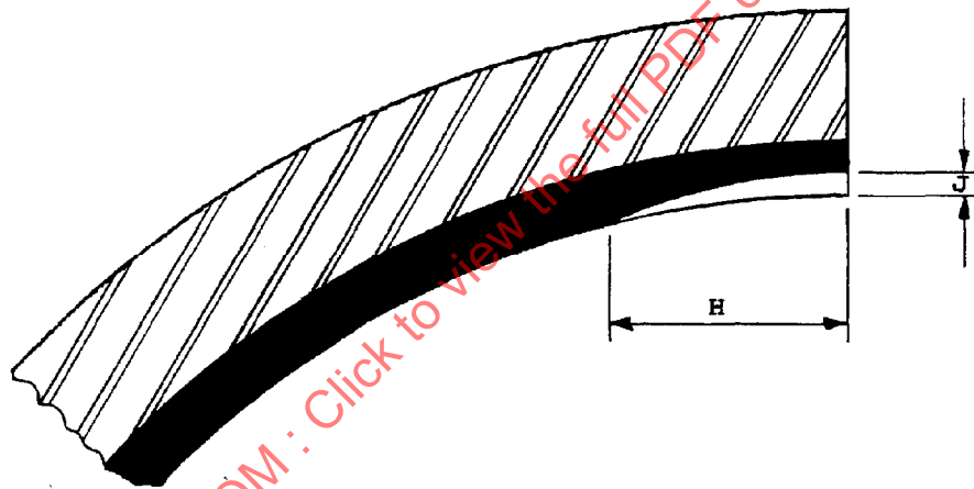
FIGURE 7—PARTING LINE RELIEF
