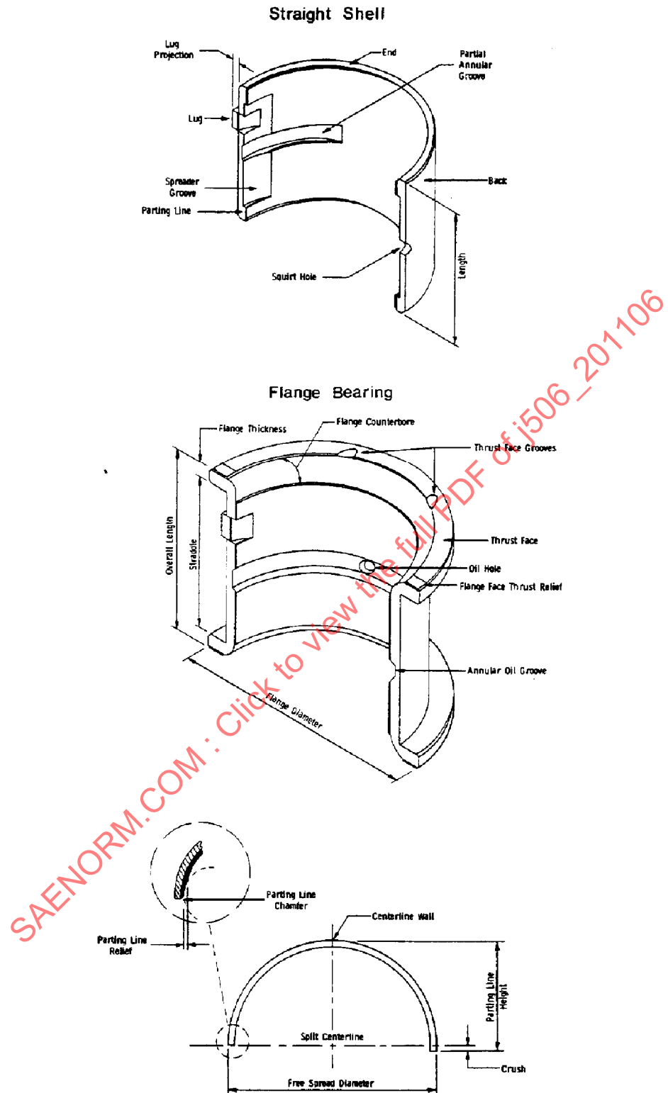
FIGURE 1—ILLUSTRATION OF COMMON BEARING CHARACTERISTICS AND TERMINOLOGY
