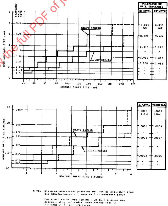
FIG. 2—BEARING WALL THICKNESS RECOMMENDATIONS
