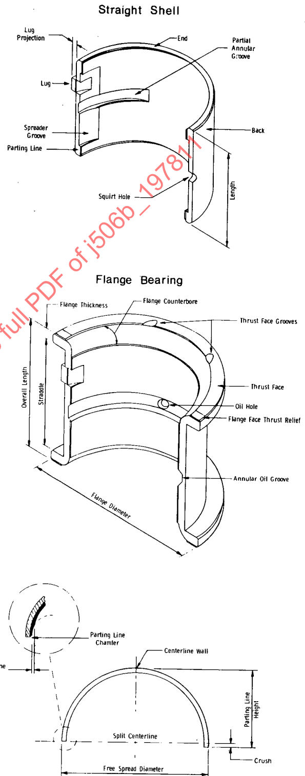
FIG. 1—ILLUSTRATION OF COMMON BEARING CHARACTERISTICS AND TERMINOLOGY
