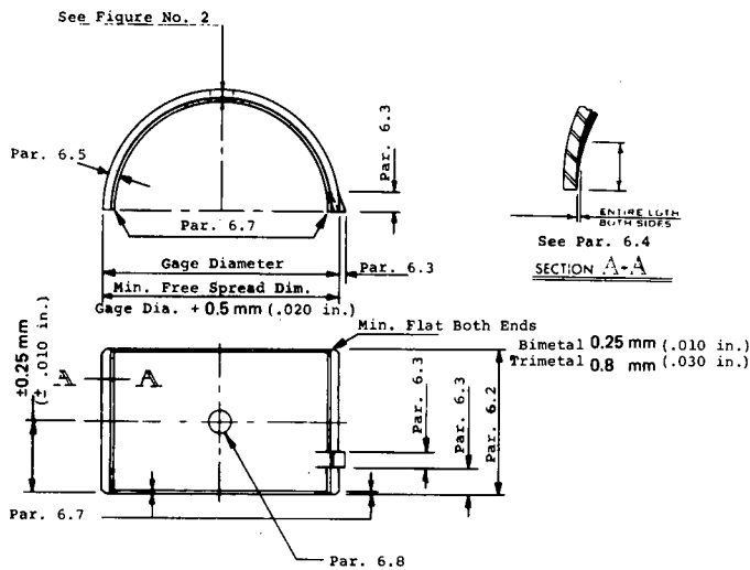
FIG. 3—STANDARD TOLERANCES OF STRAIGHT SHELL BEARINGS
