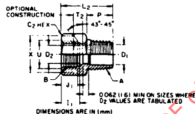
Ø FIGURE 29 - Internal Flare To External Pipe Reducing Adaptor (010106) (U5)
