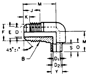
Ø FIGURE 25 - Flare To Solder 90 Deg Reducing Elbow (010204) (ES)
