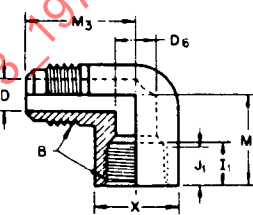
Ø FIGURE 15 - Internal Flare To External Flare 90 Deg Elbow (010205) (E4)
