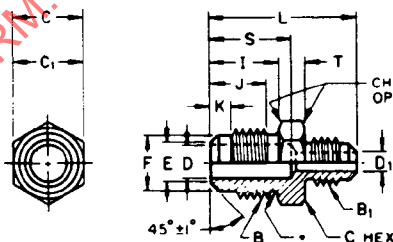
FIGURE 21 - Reducing Union (010101) (UR2)
