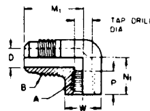
FIGURE 32 - 90 Deg Internal Pipe Thread Reducing Elbow (010203) (E3)
