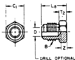
FIGURE 10 - Plug (010109) (P2)
