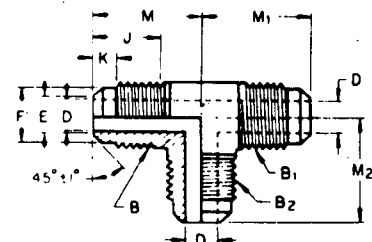
FIGURE 33 - Three-Way Reducing Tee (010401) (TR2)
