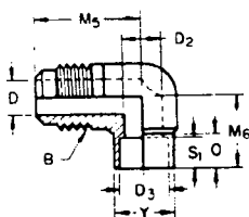
Ø FIGURE 16 - 90 Deg Solder Elbow (010204) (E5)
