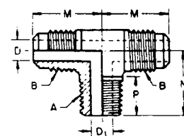
Ø FIGURE 18 - Two Way Tee (010425) (T1)
