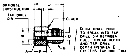
Ø FIGURE 28 - Internal Thread Reducing Connector (Half Union) (010103) (U3)
