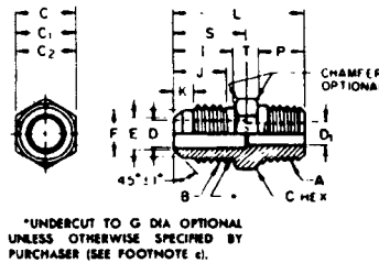
Ø FIGURE 26 - Reducing Connector (Half Union) (010102) (U1)
