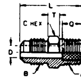
Ø FIGURE 27 - Fusible Reducing Connector (Half Union) (010163) (FU)
