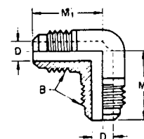
FIGURE 12 - 90 Deg Elbow Union (010201) (E2)
