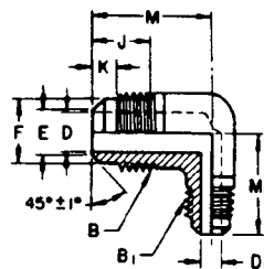
Ø FIGURE 24 - Flare To Solder Reducing Connector (Half Union) (010104) (US3)
