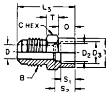
FIGURE 5 - Solder Connector (Half Union) (010104) (US3)
