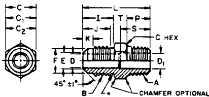
FIGURE 1 - Connector (Half Union) (010102) (U1)
