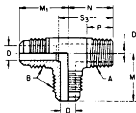
Ø FIGURE 19 - Right Angle Two Way Tee (010424) (T3)
