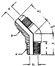
FIGURE 31 - 45 Deg Reducing Elbow (010302) (E5)
