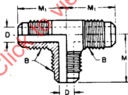
Ø FIGURE 17 - Three Way Tee (010401) (T2)
