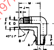
Ø FIGURE 30 - 90 DEG. Reducing Elbow (010202) (E1)
