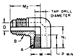
Ø FIGURE 14 - 90 Deg Internal Pipe Thread Elbow (010203) (E3)
