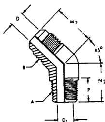
Ø FIGURE 13 - 45 Deg Elbow (010302) (E5)
