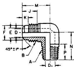
FIGURE 11 - 90 Deg Elbow (010202) (E1)
