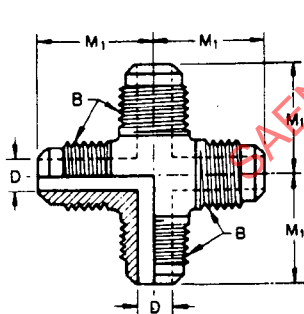
FIGURE 20 - Cross (010501) (C1)
