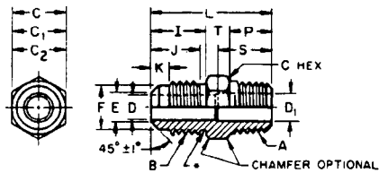
FIGURE 1 - Connector (Half Union) (010102) (U1)
