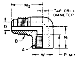
FIGURE 14 - 90 Degree Internal Pipe Thread Elbow (010203) (E3)
