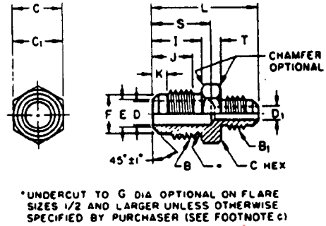
FIGURE 21—REDUCING UNION (010101) (UR2)
