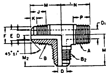
FIGURE 35—RIGHT ANGLE TWO-WAY REDUCING TEE (010424) (T3)
