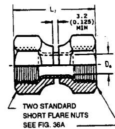
(R) FIGURE 9—INTERNAL FLARE SWIVEL UNION (010108) (US4)
