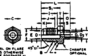
FIGURE 24—FLARE TO SOLDER REDUCING CONNECTOR (HALF UNION) (010104) (US3)
