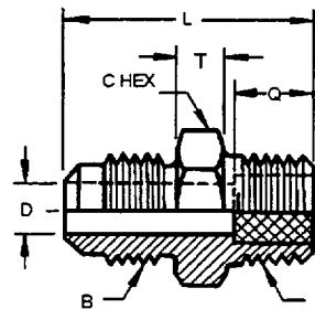
FIGURE 27—FUSIBLE REDUCING CONNECTOR (HALF UNION) (101063) (FU)
