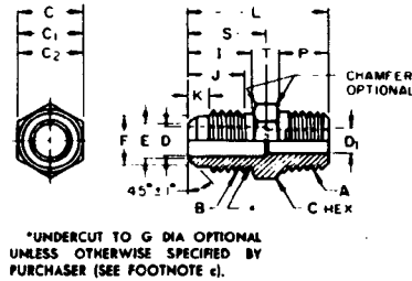
FIG. 26—REDUCING CONNECTOR (HALF UNION) (010102) (U1)
