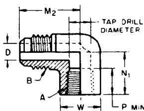
FIG. 14—90 DEG INTERNAL PIPE THREAD ELBOW (010203) (E3)
