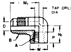
FIG. 32—90 DEG INTERNAL PIPE THREAD REDUCING ELBOW (010203) (E3)
