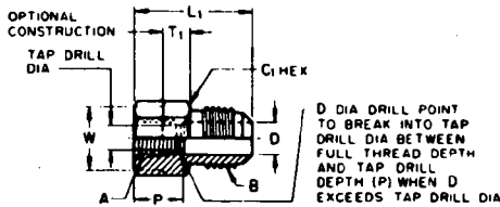
FIG. 28—INTERNAL THREAD REDUCING CONNECTOR (HALF UNION) (010103) (U3)
