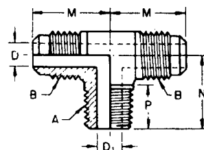
FIG. 18—TWO WAY TEE (010425) (T1)
