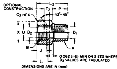
FIG. 29—INTERNAL FLARE TO EXTERNAL PIPE REDUCING ADAPTOR (010106) (U5)
