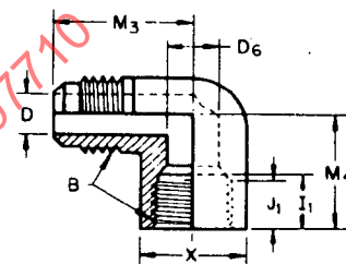
FIG. 15—INTERNAL FLARE TO EXTERNAL FLARE 90 DEG ELBOW (010205) (E4)
