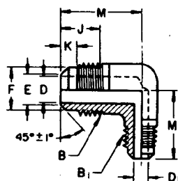
FIG. 23—90 DEG REDUCING ELBOW UNION (010201) (ER2)
