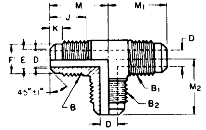
FIG. 33—THREE-WAY REDUCING TEE (010401) (TR2)
