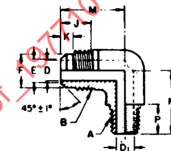
FIG. 30—90 DEG REDUCING ELBOW (010202) (E1)
