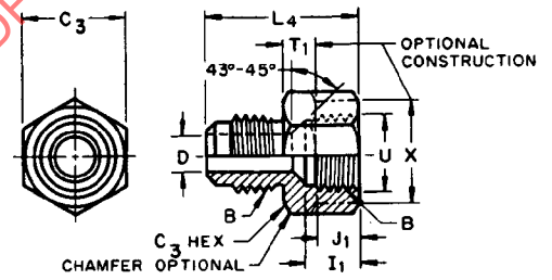
FIG. 6—INTERNAL FLARE TO EXTERNAL FLARE ADAPTOR (010105) (UR3)
