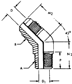
FIG. 31—45 DEG REDUCING ELBOW (010302) (E5)
