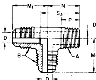
FIG. 19—RIGHT ANGLE TWO WAY TEE (010424) (T3)
