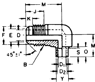
FIG. 25—FLARE TO SOLDER 90 DEG REDUCING ELBOW (010204) (ES)
