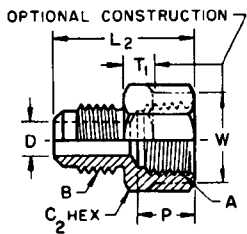
FIG. 4—INTERNAL PIPE THREAD CONNECTOR (HALF UNION) (010103) (U3)
