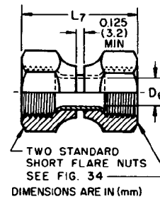
FIG. 9—INTERNAL FLARE SWIVEL UNION (010108) (US4)
