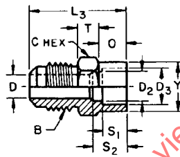
FIG. 5—SOLDER CONNECTOR (HALF UNION) (010104) (US3)
