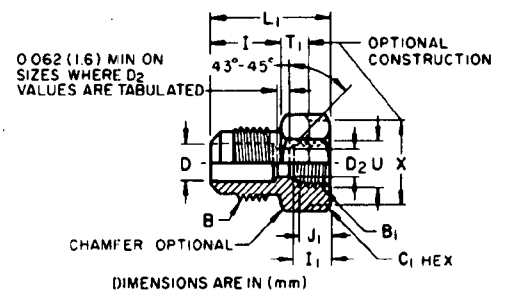
FIG. 22—INTERNAL FLARE TO EXTERNAL FLARE REDUCING ADAPTOR (010105) (UR3)
