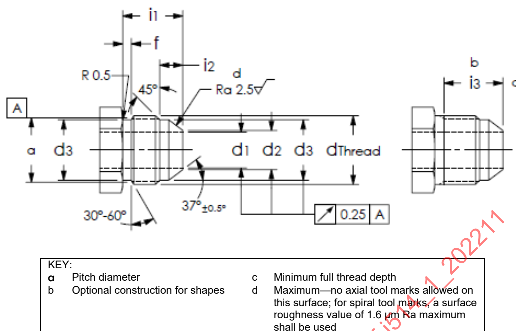
Figure 8 - 37 degree flared connection
