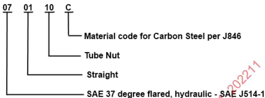
Figure 5 - Connector style designation with material modifier
