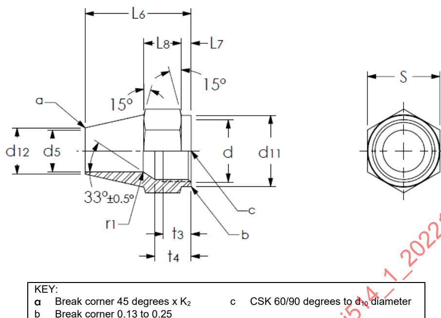
Figure 11 - Long tube nut (070111, 07M0111)
