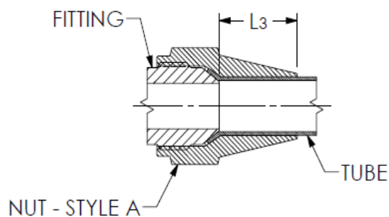
Figure 7B - Two piece tube assembly – Long Nut
