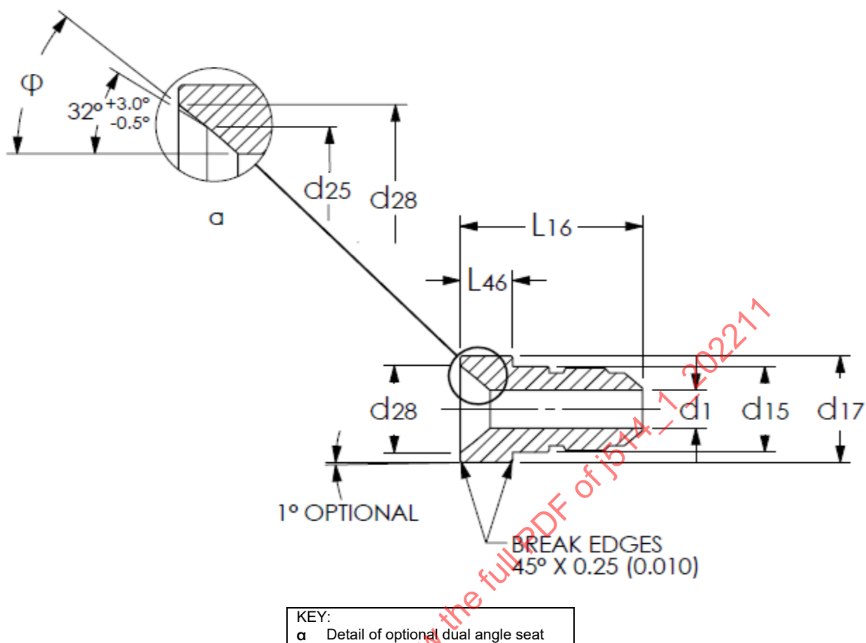
Figure 15 - Reducing adapter (070123) (1)(2)
