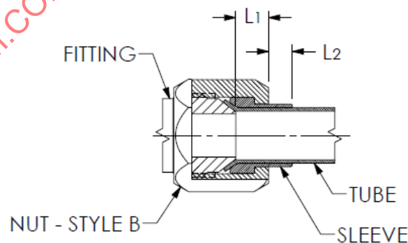
Figure 7A - Three piece tube assembly - Short Nut
