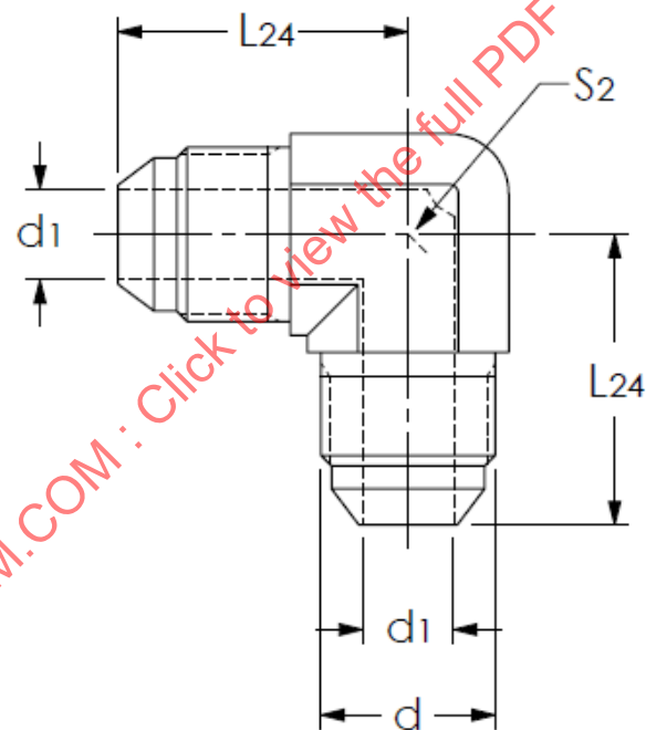
Figure 33 - 90 degree union elbow (070201, 07M0201)
