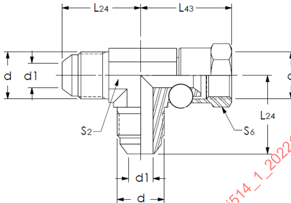
Figure 38 - Swivel run tee (070432, 07M0432)
