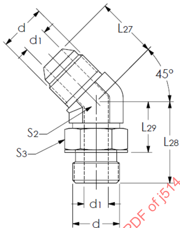
Figure 20 - 45 degree straight thread elbow (070320, 07M0320)
