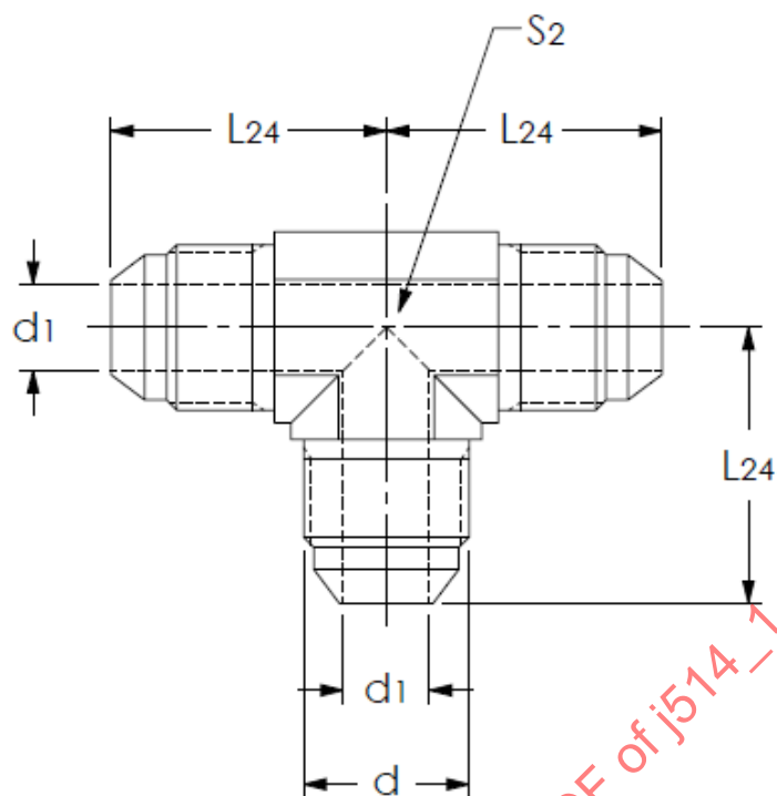
Figure 34 - Union tee (070401, 07M0401)
