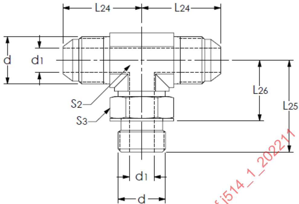
Figure 22 - Straight thread branch tee (070429, 07M0429)
