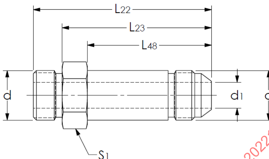
Figure 18 - Straight thread connector - Long (071720, 07M1720)
