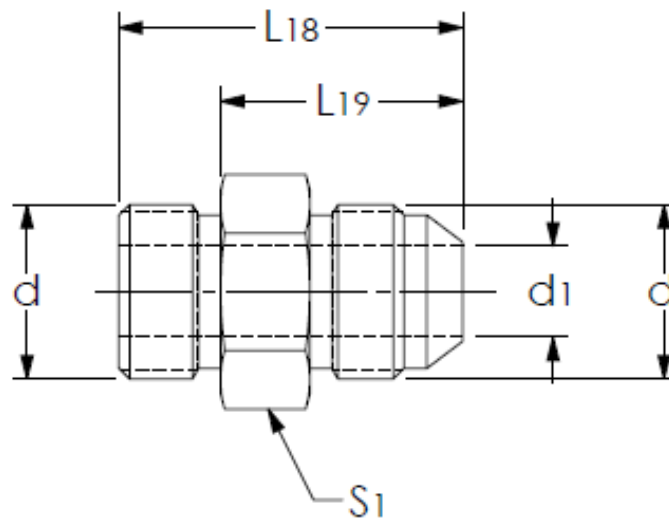
Figure 16 - Straight thread connector short (070120, 07M0120)
