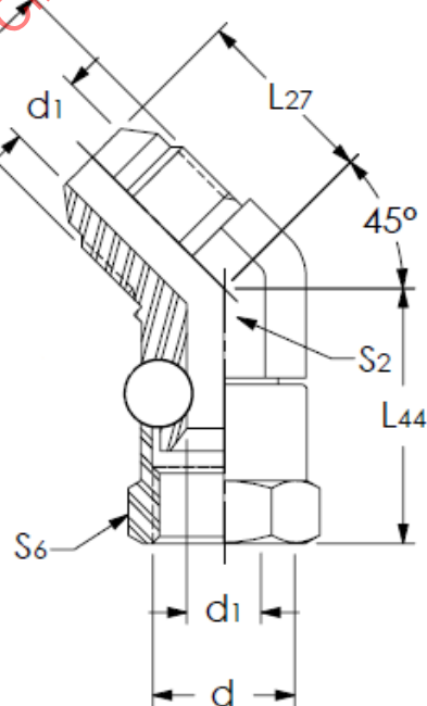
Figure 37 - 45 degree swivel elbow (070321, 07M0321)
