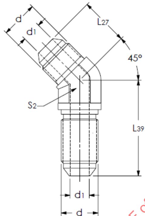
Figure 29 - 45 degree bulkhead elbow (070801, 07M0801)
