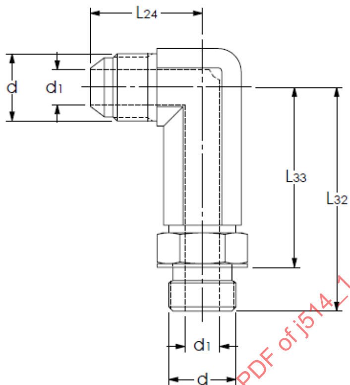
Figure 24 - 90 degree straight thread elbow, extra long (071620, 07M1620)
