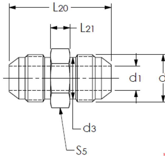
Figure 32 - Union (070101, 07M0101)
