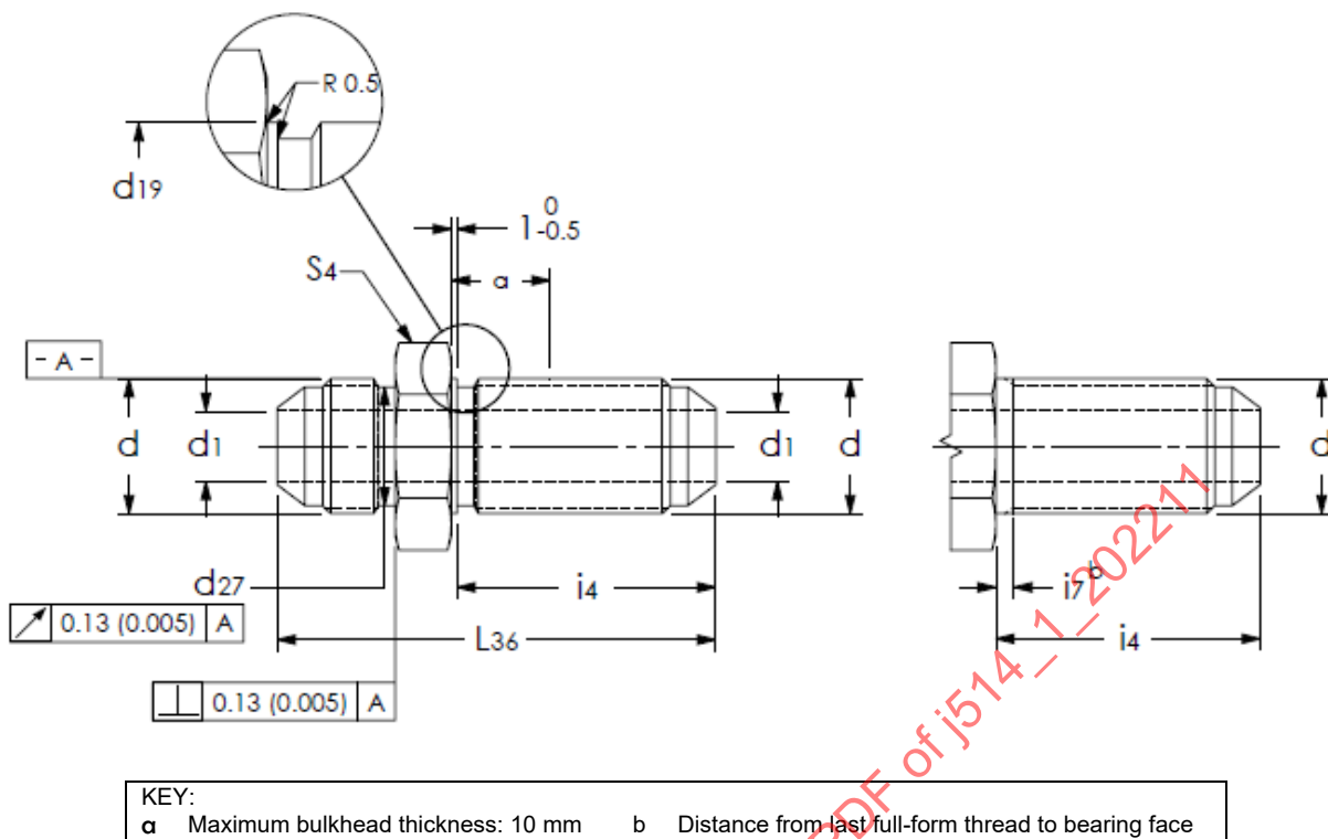
Figure 27 - Bulkhead union (070601, 07M0601), optional construction
