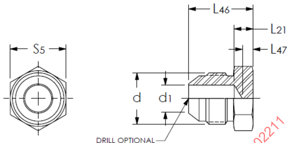
Figure 14 - Plug (070109, 07M0109)
