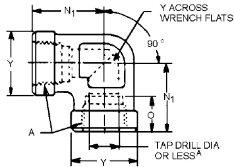
Figure 8 - 90 degree pipe elbow (140238)
