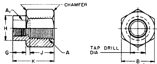
FIGURE 7—REDUCER COUPLING (130138)
