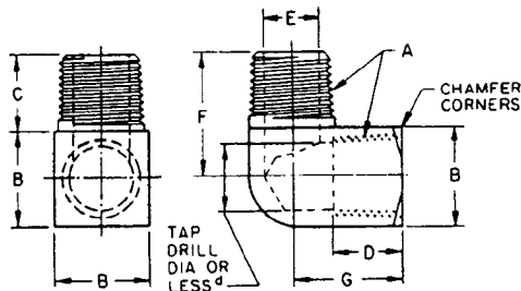
EMSFIGURE 13—90 DEGREE EMSSTREET ELBOW (130239)
