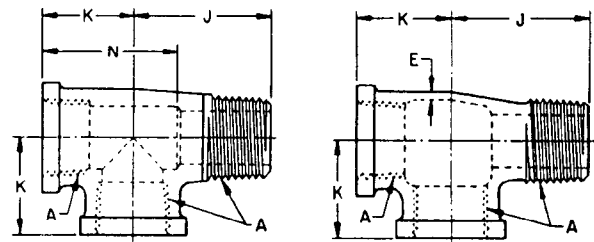
FIGURE 12C—INTERNAL, EXTERNAL, INTERNAL TEES (130424)
