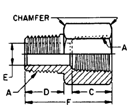
FIGURE 3—ADAPTER (130139)
