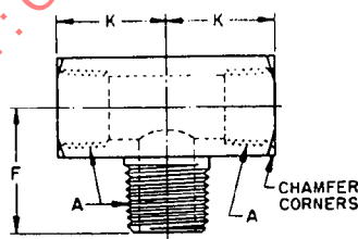
FIGURE 17B—INTERNAL, INTERNAL, EXTERNAL (130425)
