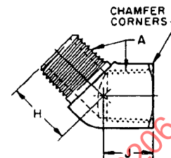
FIGURE 14—45 DEGREE STREET ELBOW (130339)
