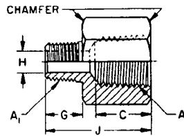
FIGURE 4—REDUCER ADAPTER (130139)
