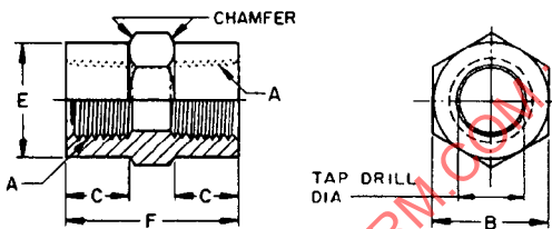
FIGURE 6—COUPLING (130138)
