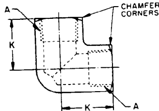
EMSFIGURE 15—90 DEGREE EMSPIPE ELBOW (130238)
