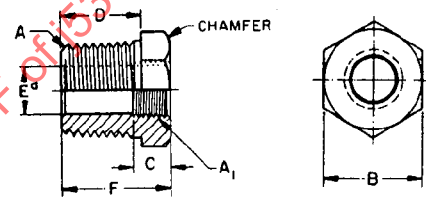
FIGURE 2—HEXAGON REDUCER NIPPLE (130137)
