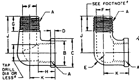
FIGURE 8—90 DEGREE STREET ELBOWS (130239)
