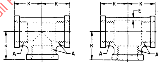
FIGURE 12A—INTERNAL, INTERNAL, INTERNAL TEES (130438)
