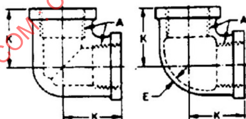
Figure 10 - 90-degree pipe elbows (130238)
