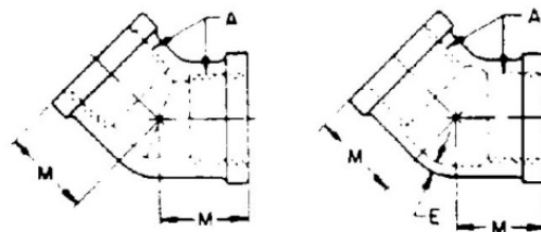
Figure 11 - 45-degree pipe elbows (130338)
