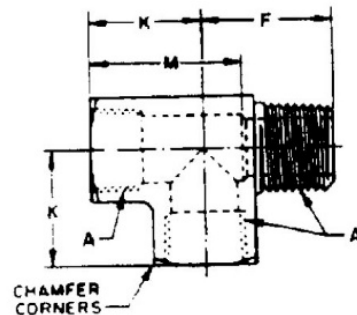
Figure 17C - Internal, external, internal (130424)
