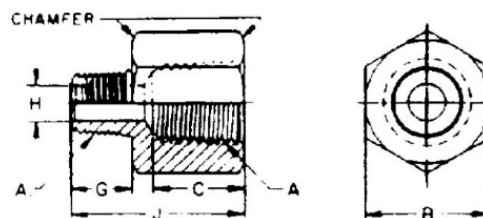
Figure 4 - Reducer adapter (130139)
