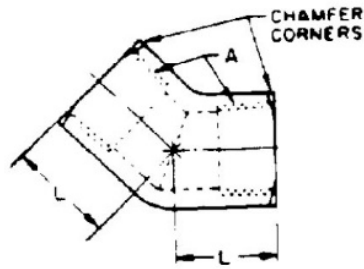
Figure 16 - 45-degree pipe elbow (130338)
