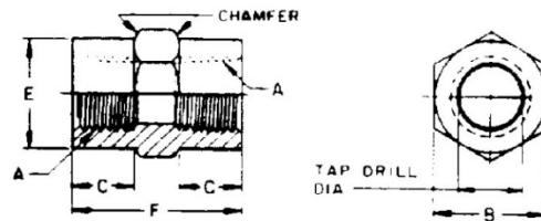
Figure 6 - Coupling (130138)
