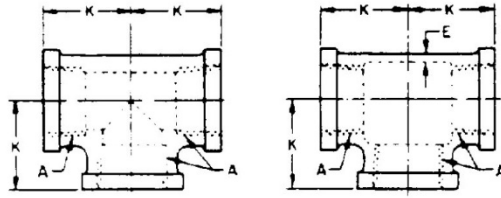
Figure 12A - Internal, internal, internal tees (130438)
