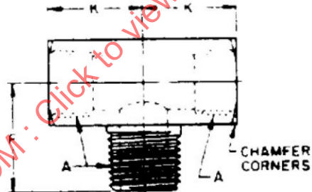
Figure 17B - Internal, internal, external (130425)
