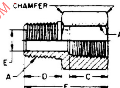
Figure 3 - Adapter (130139)
