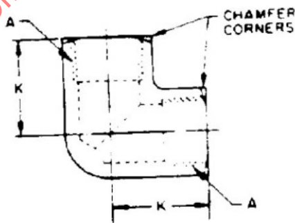
Figure 15 - 90-degree pipe elbow (130238)
