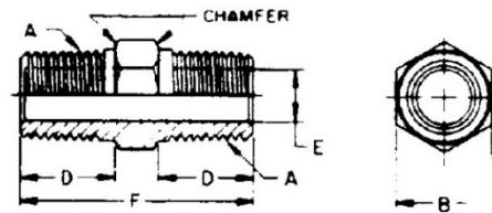
Figure 1 - Hexagon nipple (130137)
