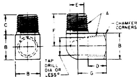
Figure 13 - 90-degree street elbow (130239)
