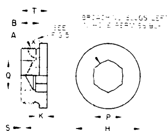
FIGURE 7B - Broached (420109H)
