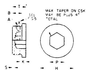
FIGURE 7C - Cast (420109J)
