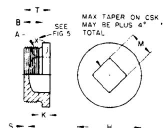
FIGURE 6C - Cast (420109F)
