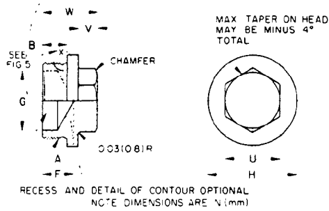
FIGURE 4 - Hexagon Inside Head Plug (420109C)
