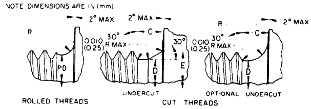
FIGURE 5 - Detail X Enlarged
