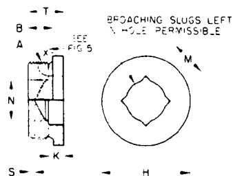
FIGURE 6B - Broached (420109E)
