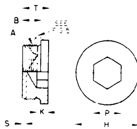
FIGURE 7A - Upset (420109G)
