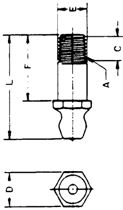
FIGURE 2C—1/4-28 TAPER THREAD
