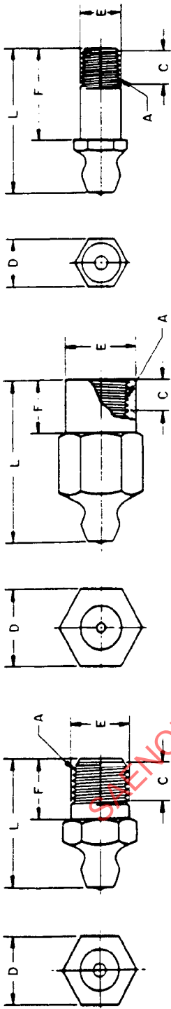
FIGURE 2A—EXTERNAL TAPER PIPE THREAD
