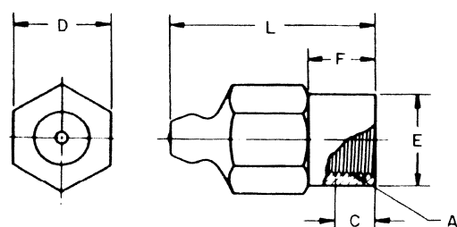
FIGURE 2B—INTERNAL TAPER PIPE THREAD
