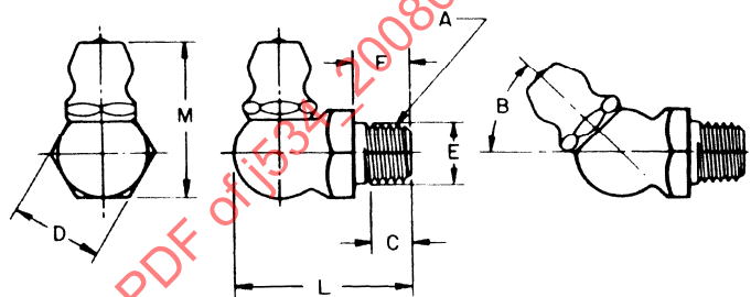
FIGURE 3B—1/4-28 TAPER THREAD
