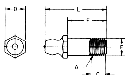
FIGURE 2C—1/4-28 TAPER THREAD
