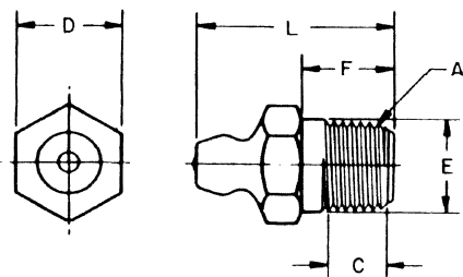
FIGURE 2A—EXTERNAL TAPER PIPE THREAD
