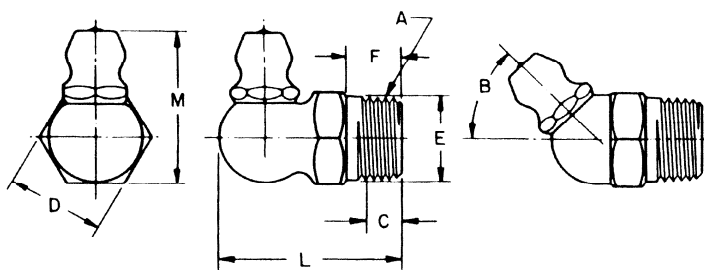
FIGURE 3A—TAPER PIPE THREAD
