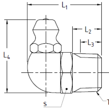
Figure 7 - 90-degree elbow fittings
