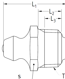
Figure 6 - Straight fittings
