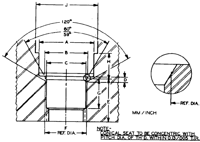
FIG. 4—HEAD COUNTERBORE—CONICAL SEAT (SEE TABLE 4)
