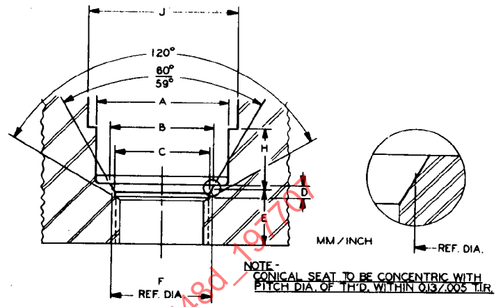
FIG. 5—HEAD COUNTERBORE—CONICAL SEAT (SPECIAL LONG REACH) (SEE TABLE 4)
