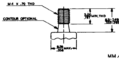
FIG. 9—THREADED POST (SEE TABLE 6)
