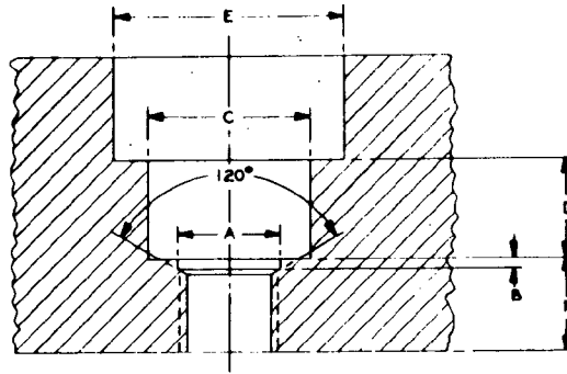
FIG. 2—HEAD COUNTERBORE—FLAT SEAT (SEE TABLE 2)
