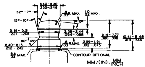
FIG. 8—ALTERNATE BANTAM SPARK PLUG SOLID POST TYPE
