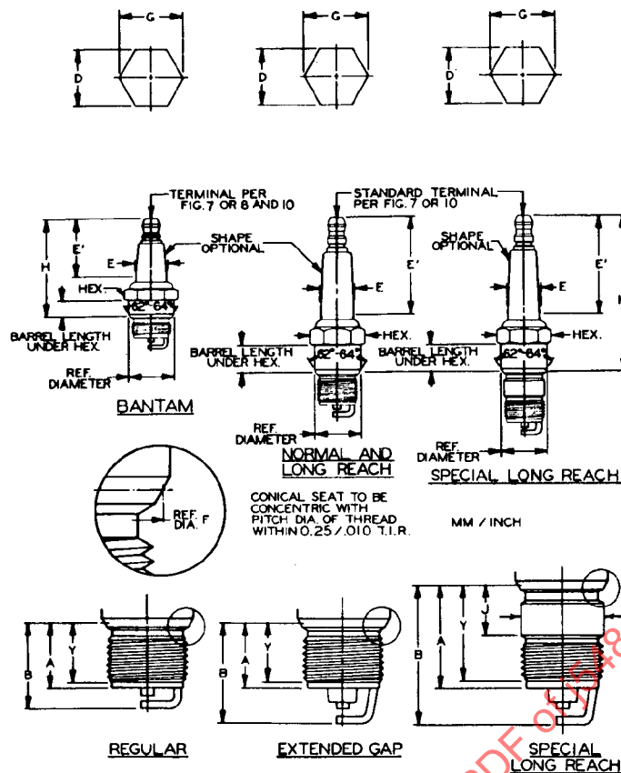
FIG. 3—CONICAL SEAT SPARK PLUGS (SEE TABLE 3)
