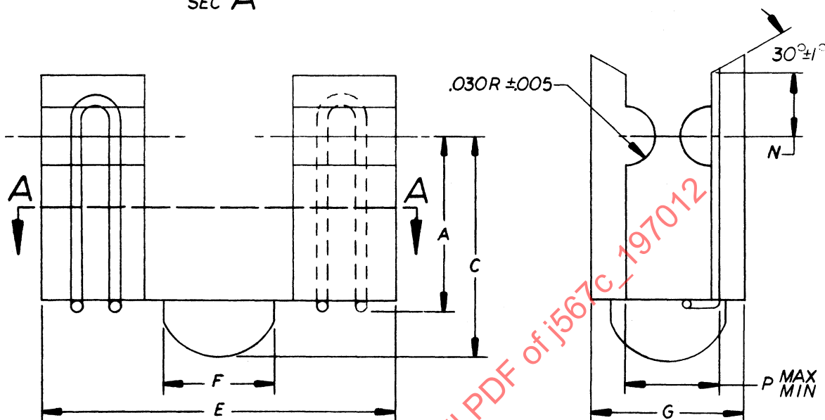
FIG. 2—WEDGE BASE GAGES
