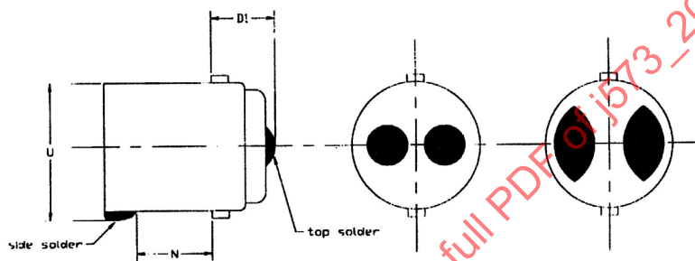
FIGURE 7B - BA15d DIMENSIONS TO BE CONTROLLED ON A FINISHED LIGHT SOURCE
