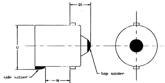
FIGURE 7A - BA15s DIMENSIONS TO BE CONTROLLED ON A FINISHED LIGHT SOURCE
