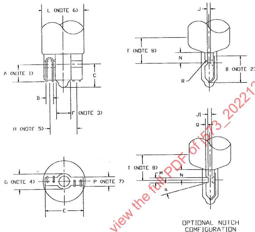
Figure 9 - Base type W2.1x9.2d
