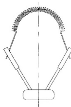
Figure 2 - Legged filament (WAA view, C-2R filament shape)
