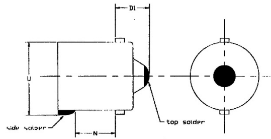
Figure 7A - BA15s base dimensions to be controlled on a finished filament light source
